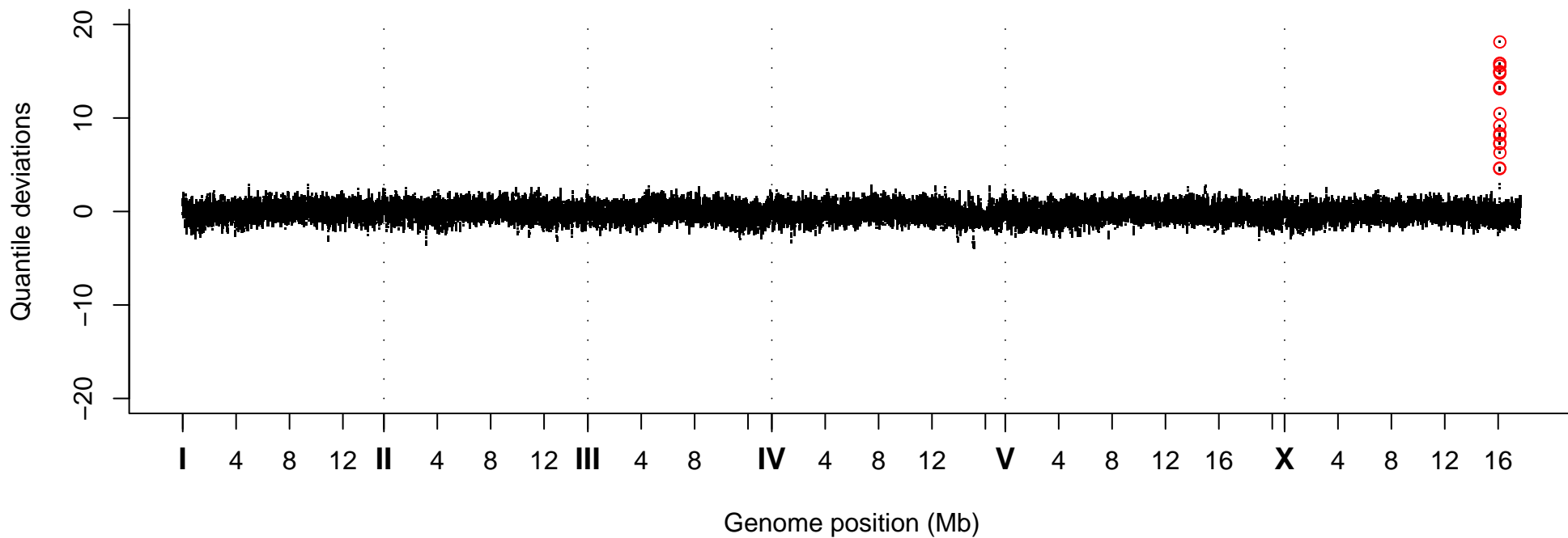
Quantile Deviations, Strain VC20685
