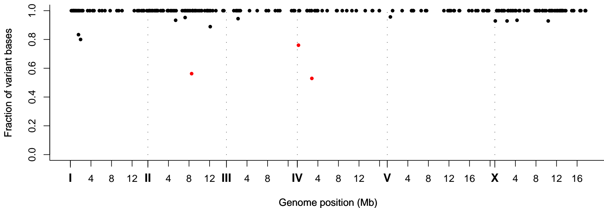
Fraction of Variant Bases at Position, Strain VC20685
