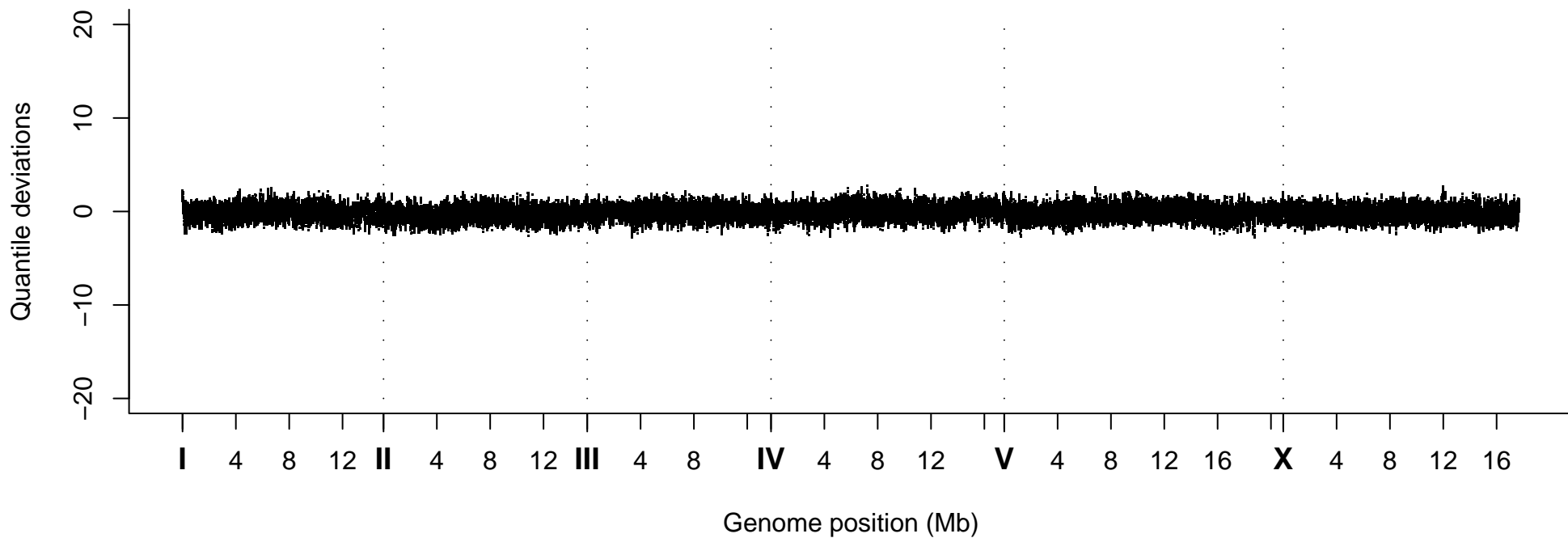
Quantile Deviations, Strain VC20691
