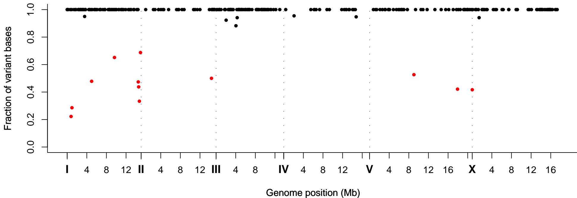
Fraction of Variant Bases at Position, Strain VC20691
