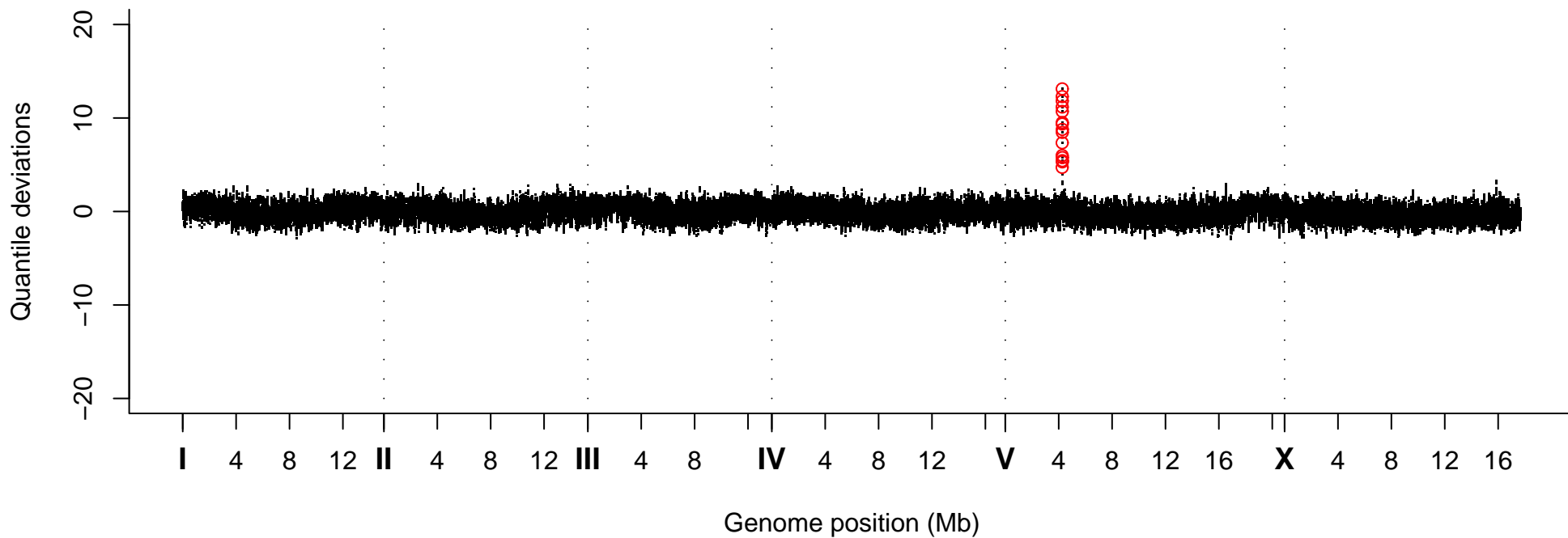
Quantile Deviations, Strain VC20703
