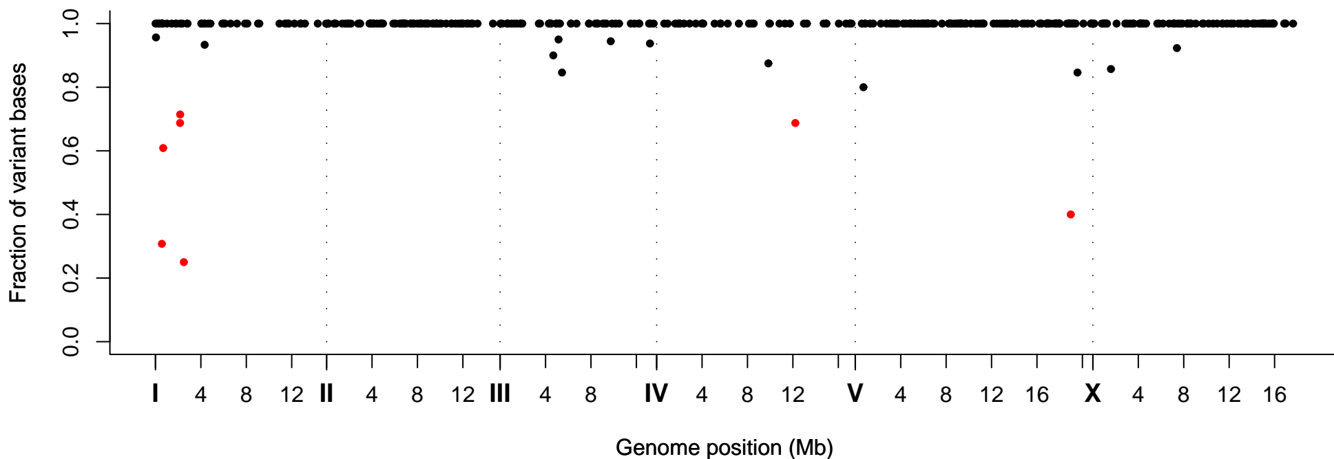
Fraction of Variant Bases at Position, Strain VC20703
