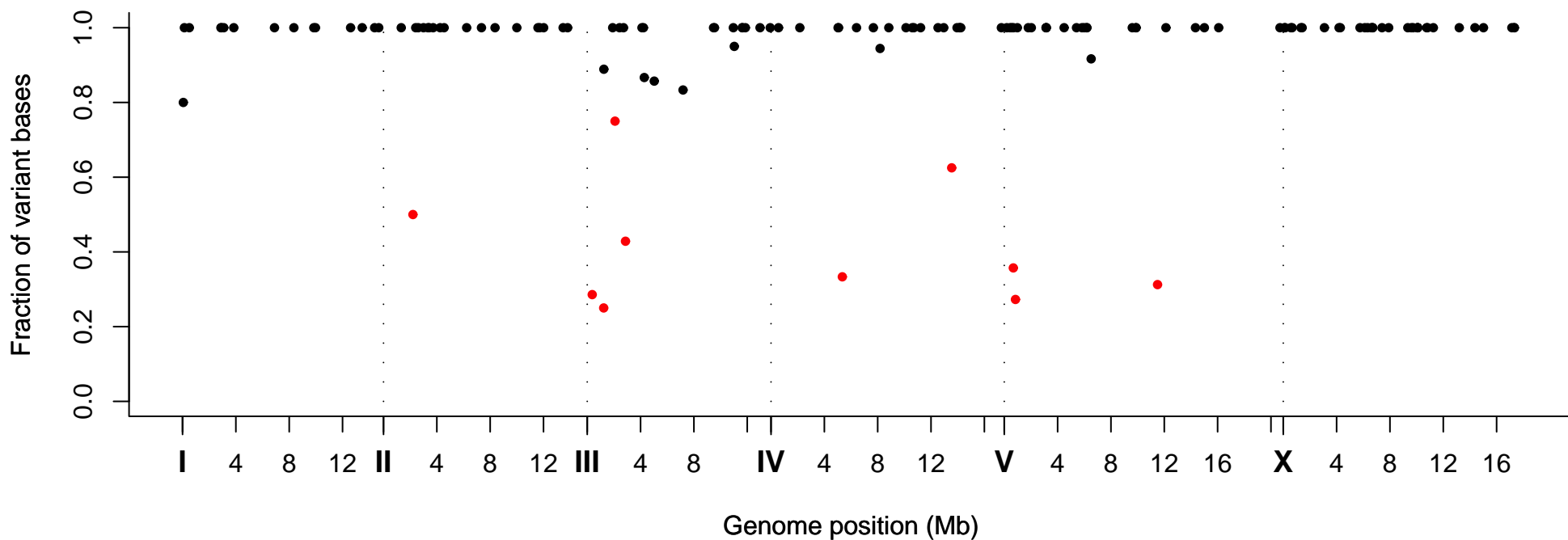
Fraction of Variant Bases at Position, Strain VC20706
