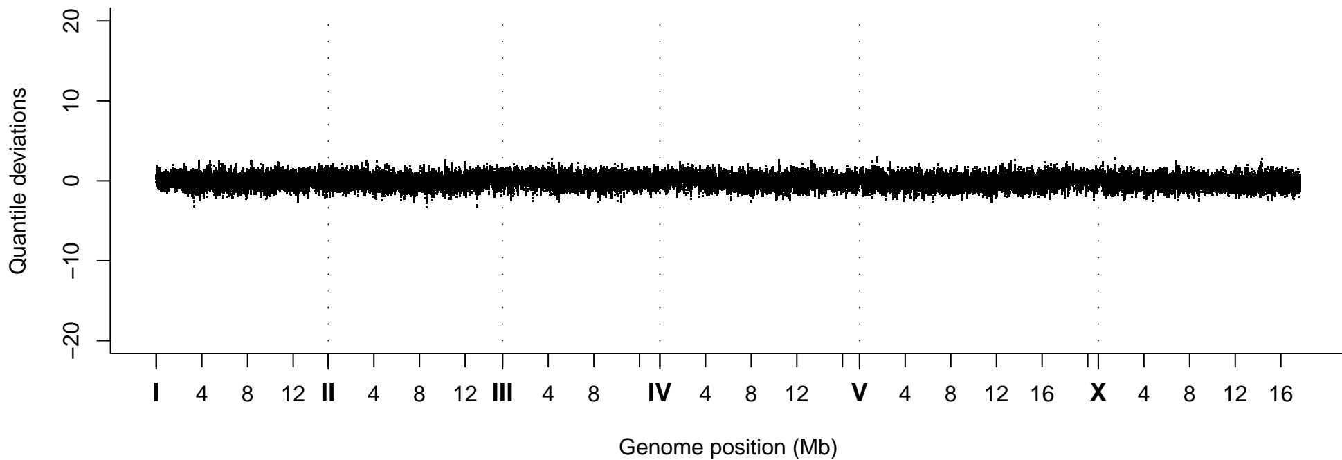
Quantile Deviations, Strain VC20706
