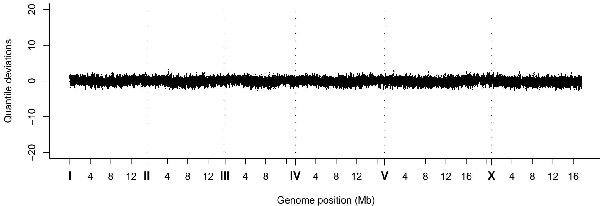
Quantile Deviations, Strain VC20707
