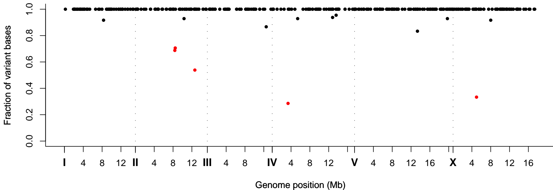
Fraction of Variant Bases at Position, Strain VC20707
