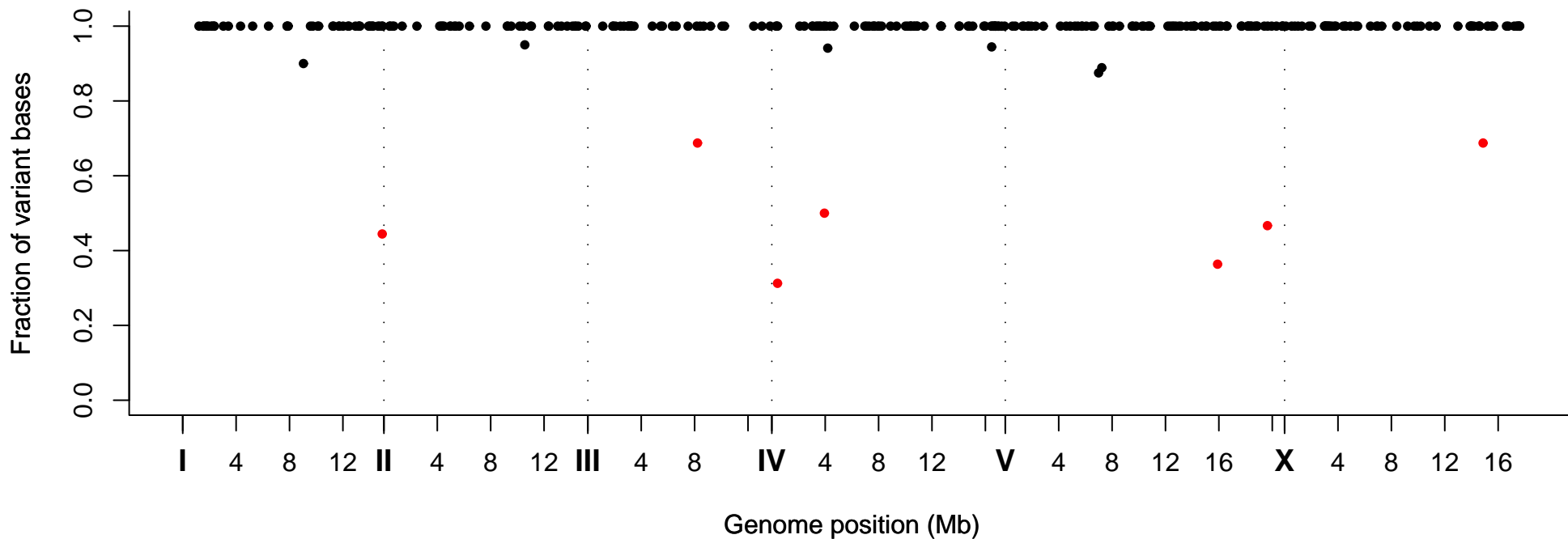
Fraction of Variant Bases at Position, Strain VC20710
