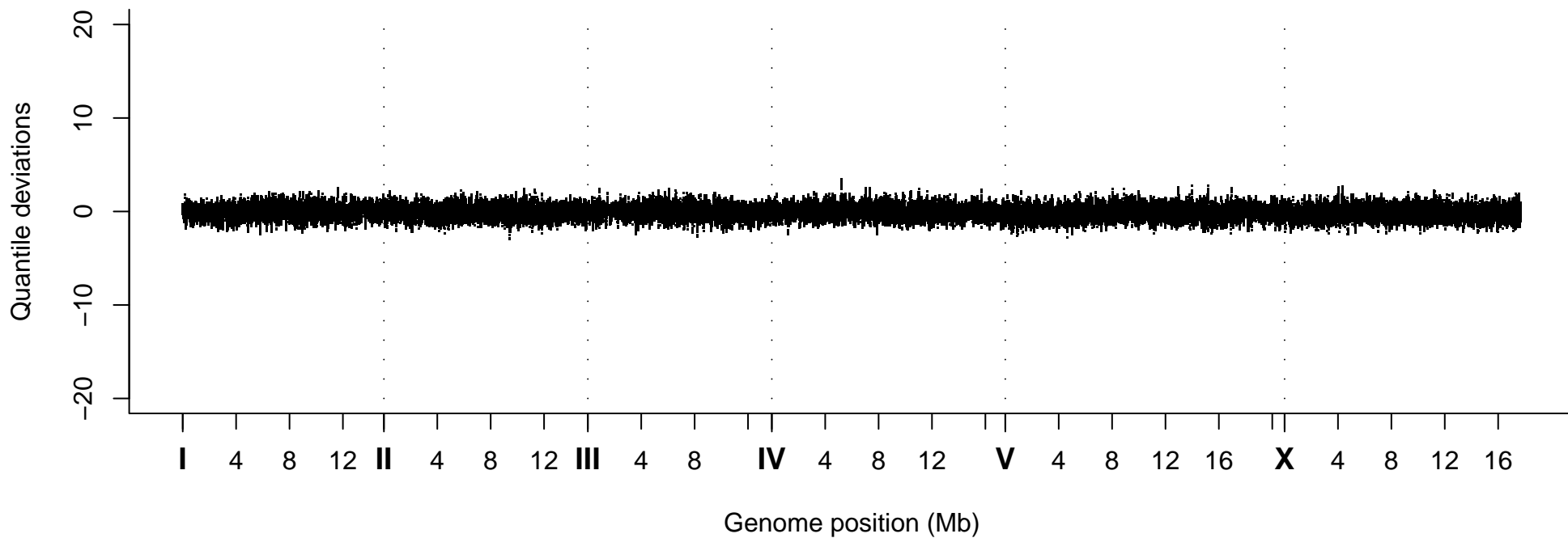
Quantile Deviations, Strain VC20710
