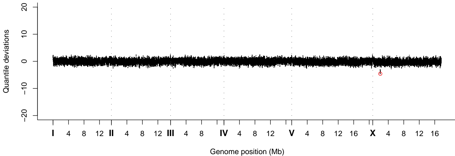
Quantile Deviations, Strain VC20711
