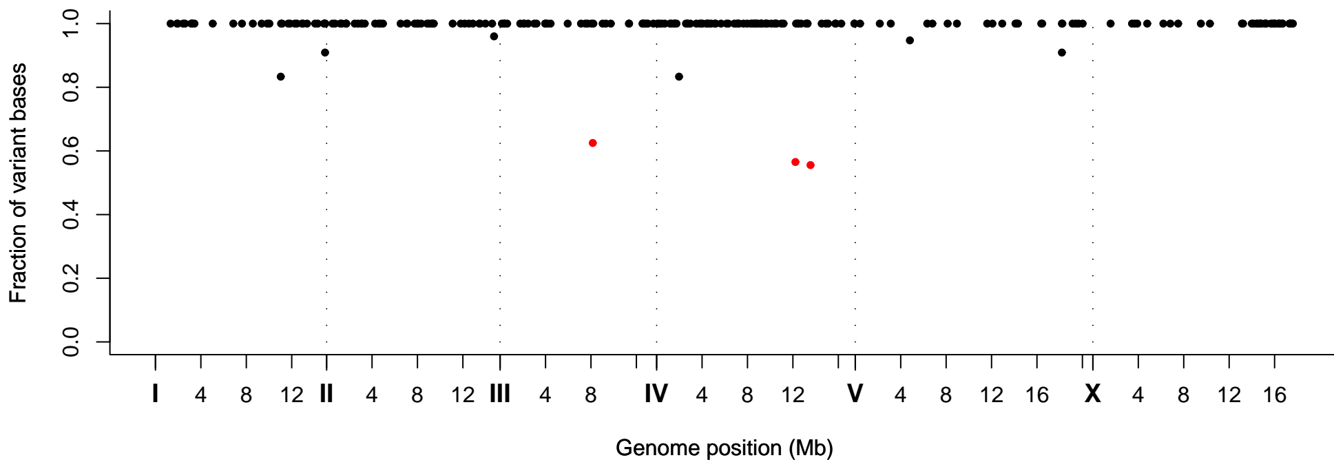
Fraction of Variant Bases at Position, Strain VC20715
