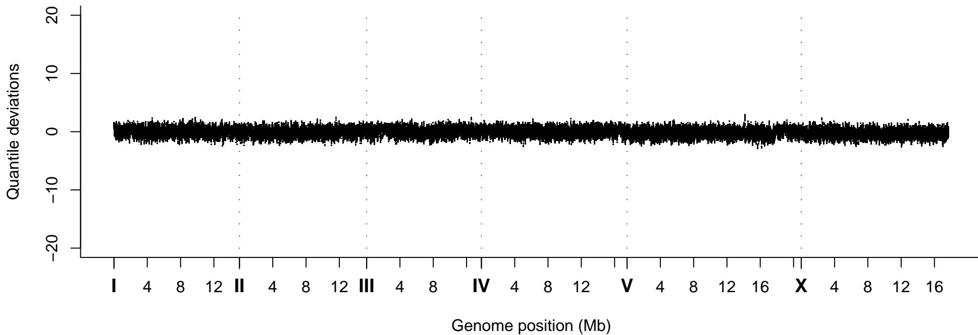
Quantile Deviations, Strain VC20715
