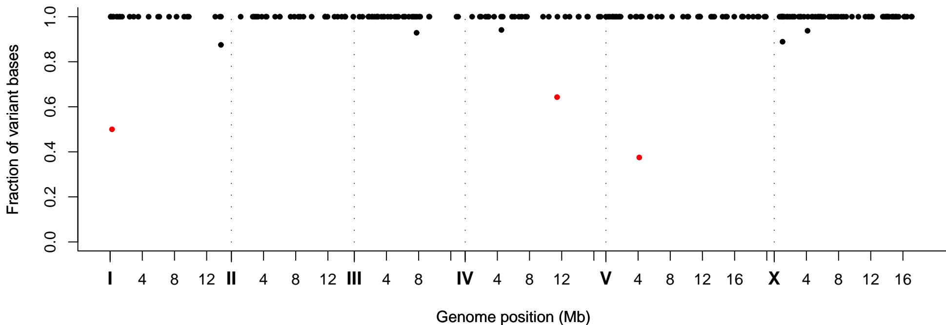
Fraction of Variant Bases at Position, Strain VC20718
