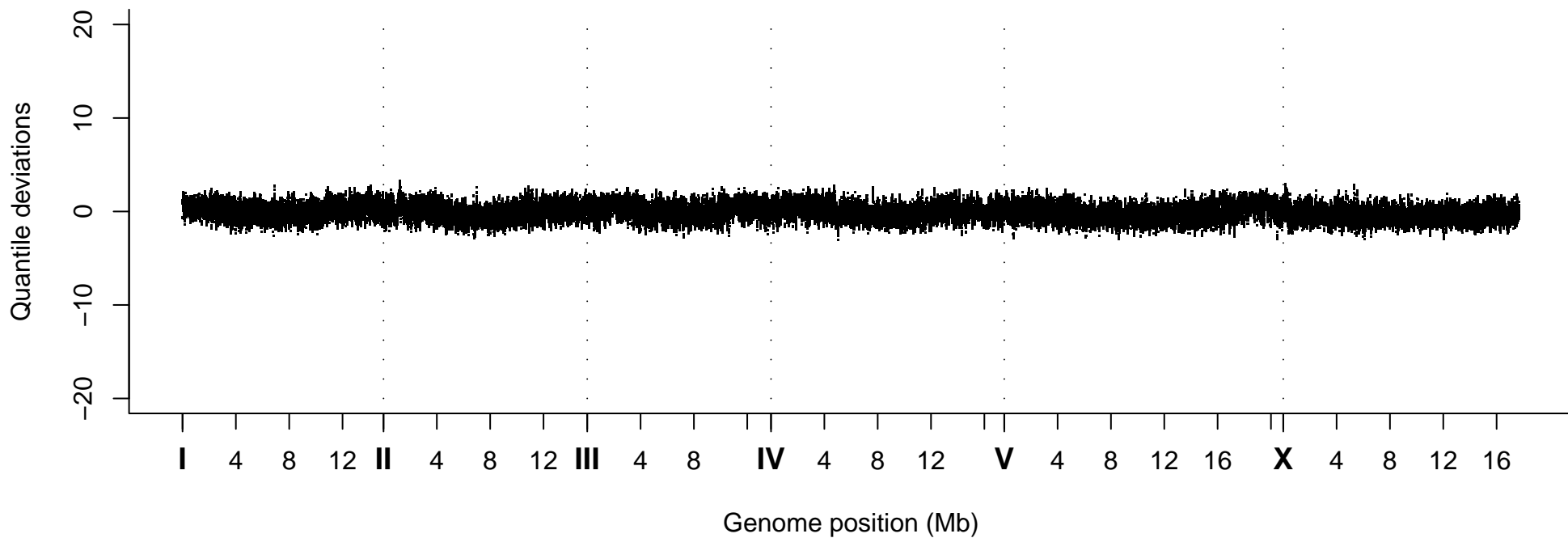
Quantile Deviations, Strain VC20721
