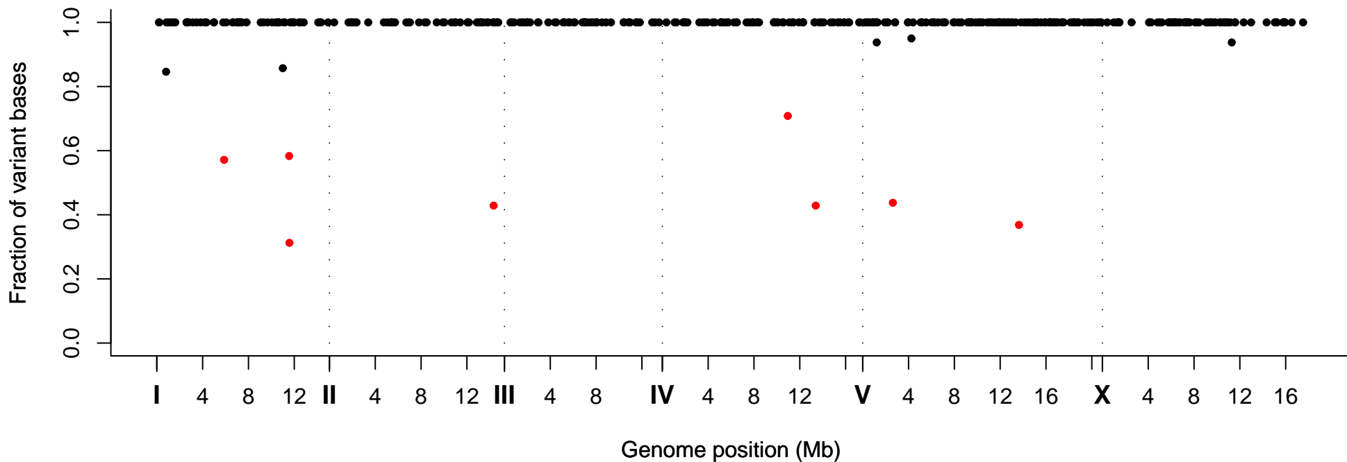
Fraction of Variant Bases at Position, Strain VC20721
