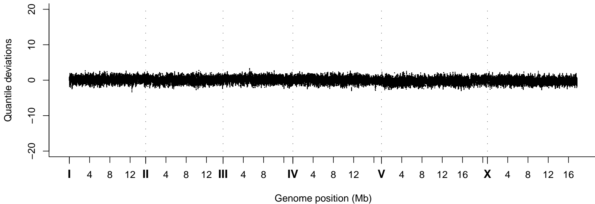
Quantile Deviations, Strain VC20724
