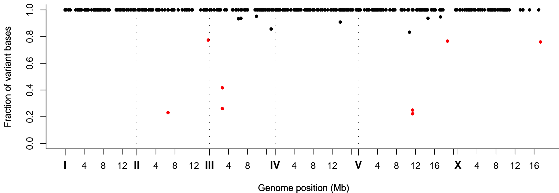
Fraction of Variant Bases at Position, Strain VC20724
