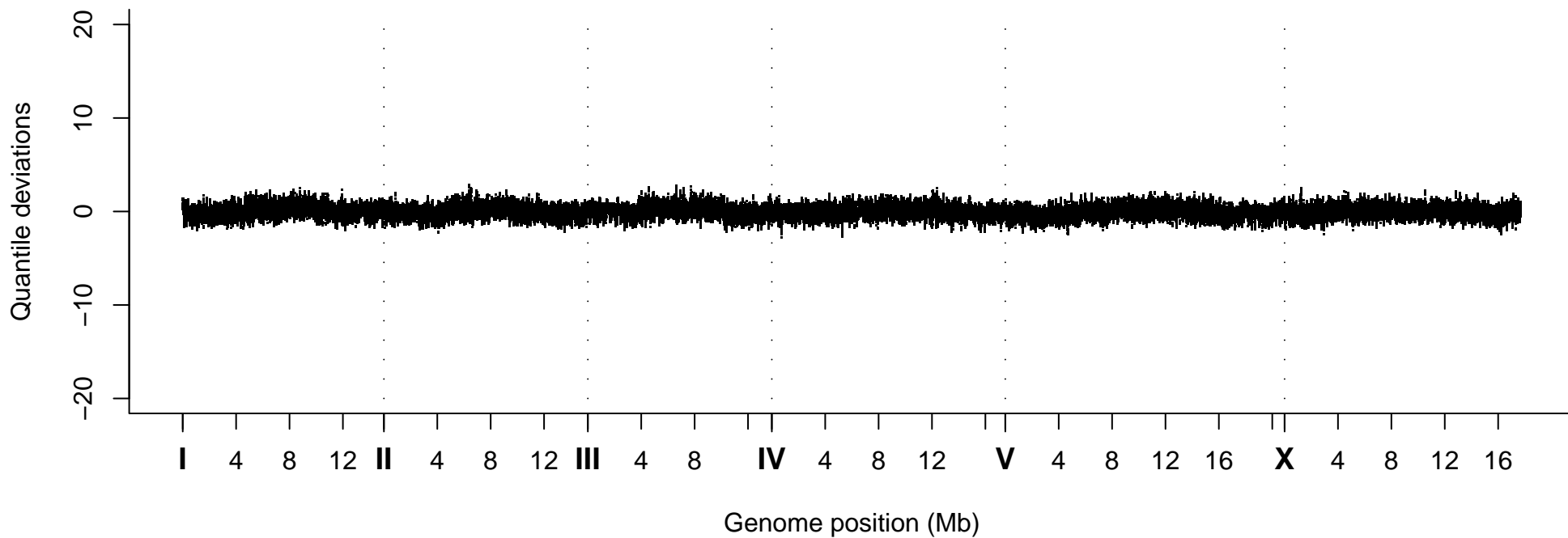
Quantile Deviations, Strain VC20741
