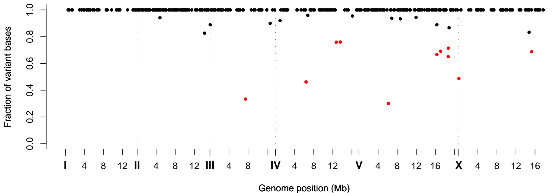
Fraction of Variant Bases at Position, Strain VC20741
