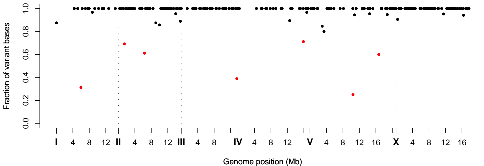
Fraction of Variant Bases at Position, Strain VC20747
