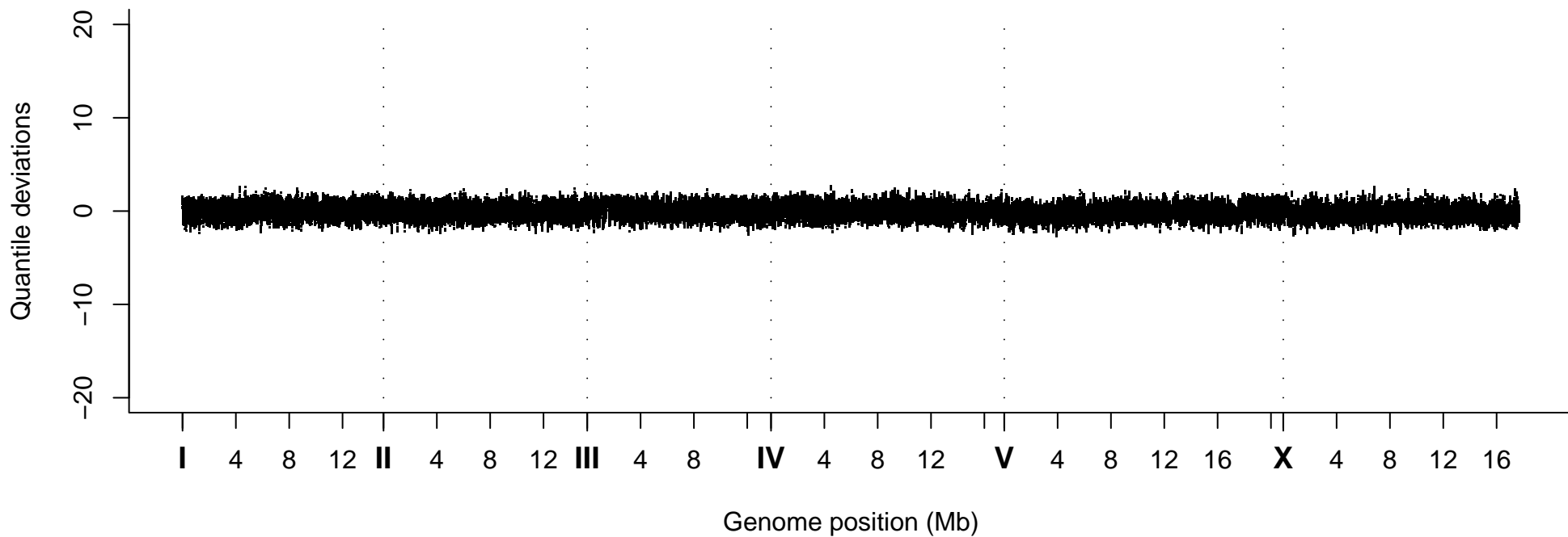
Quantile Deviations, Strain VC20747
