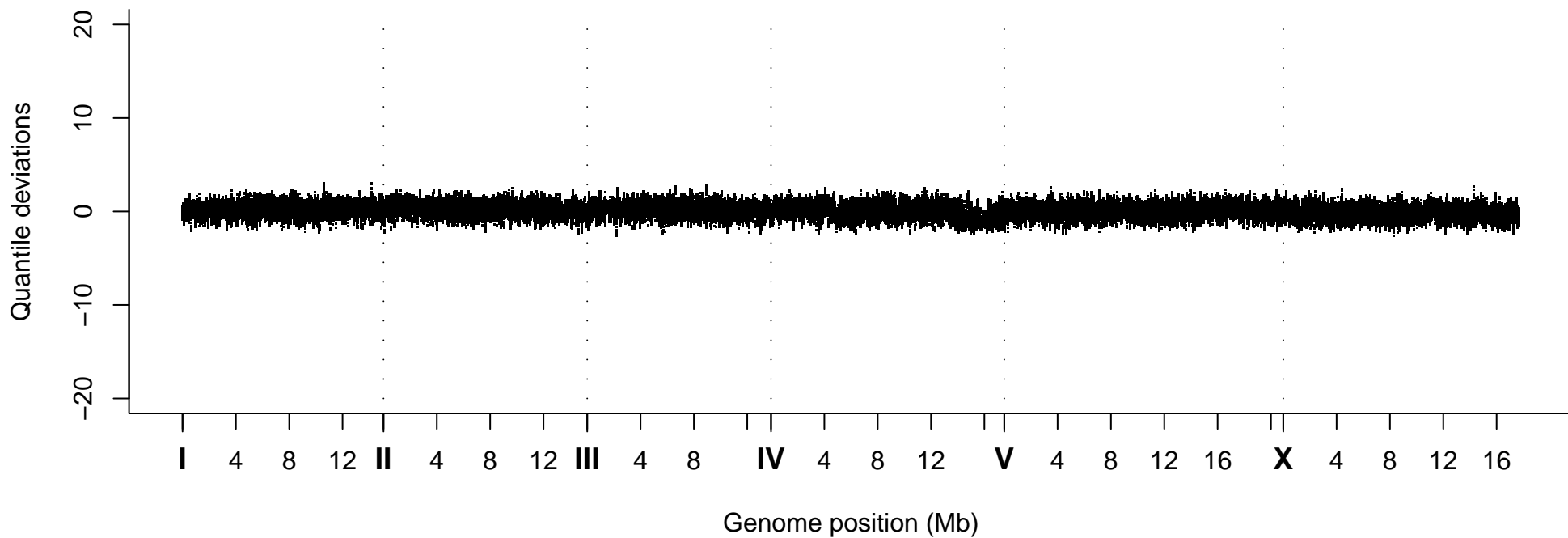
Quantile Deviations, Strain VC20749
