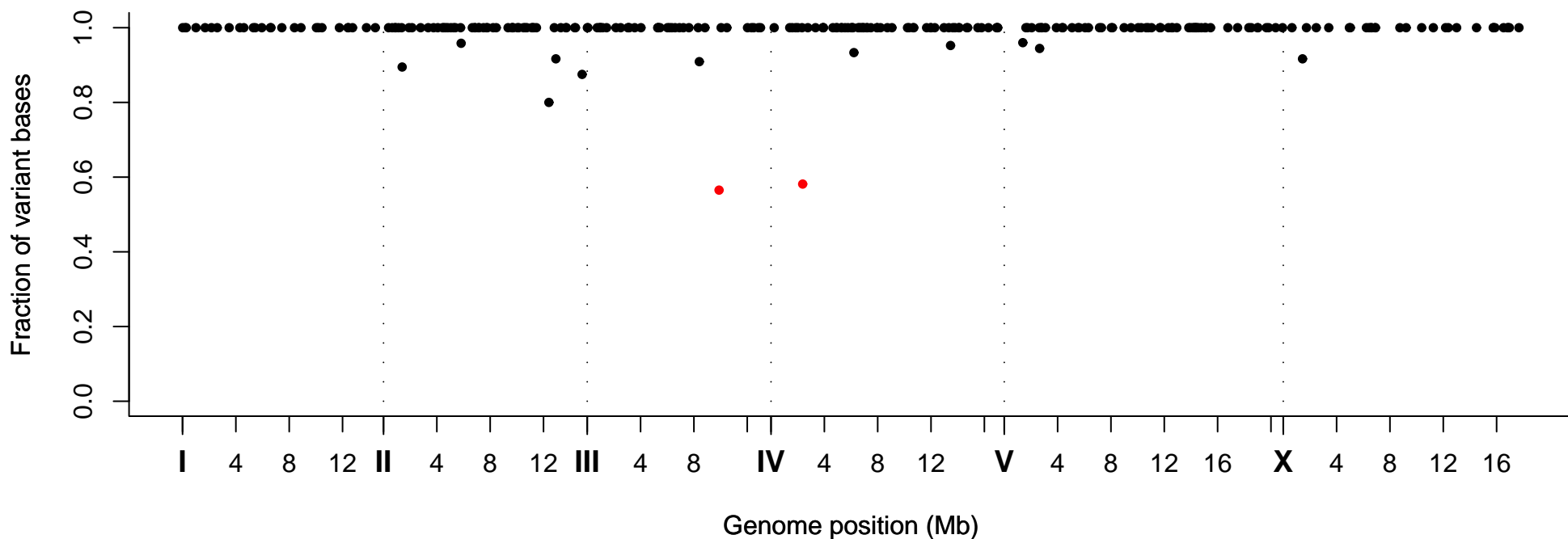
Fraction of Variant Bases at Position, Strain VC20749
