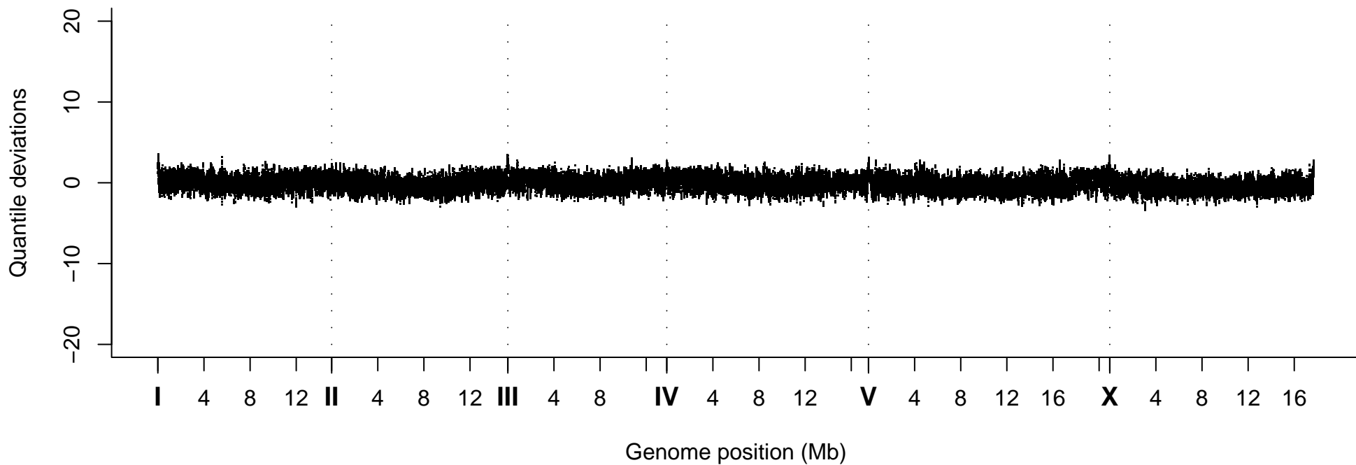
Quantile Deviations, Strain VC20762
