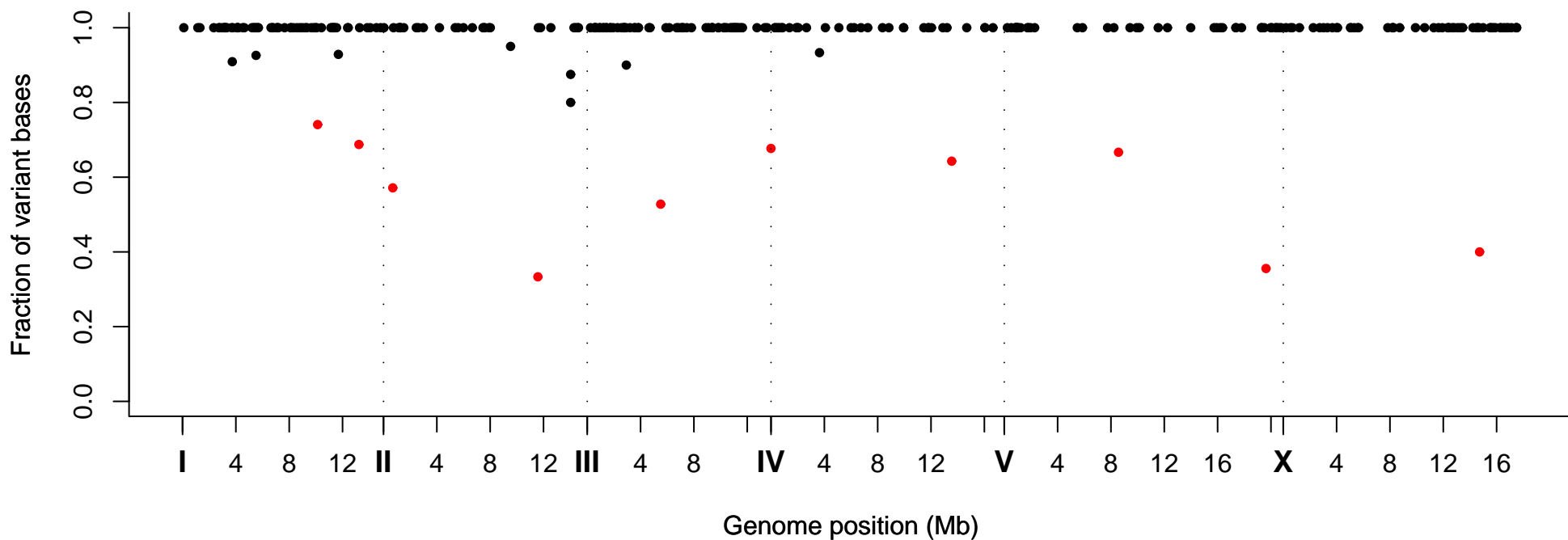
Fraction of Variant Bases at Position, Strain VC20762
