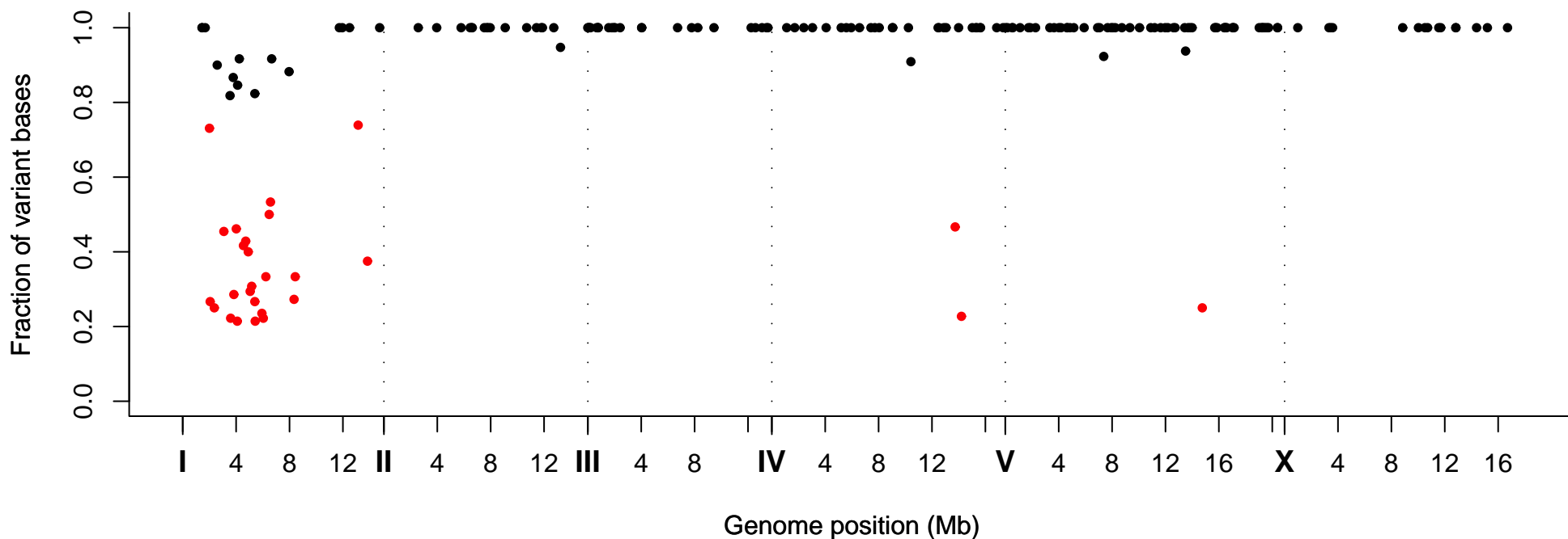
Fraction of Variant Bases at Position, Strain VC20766
