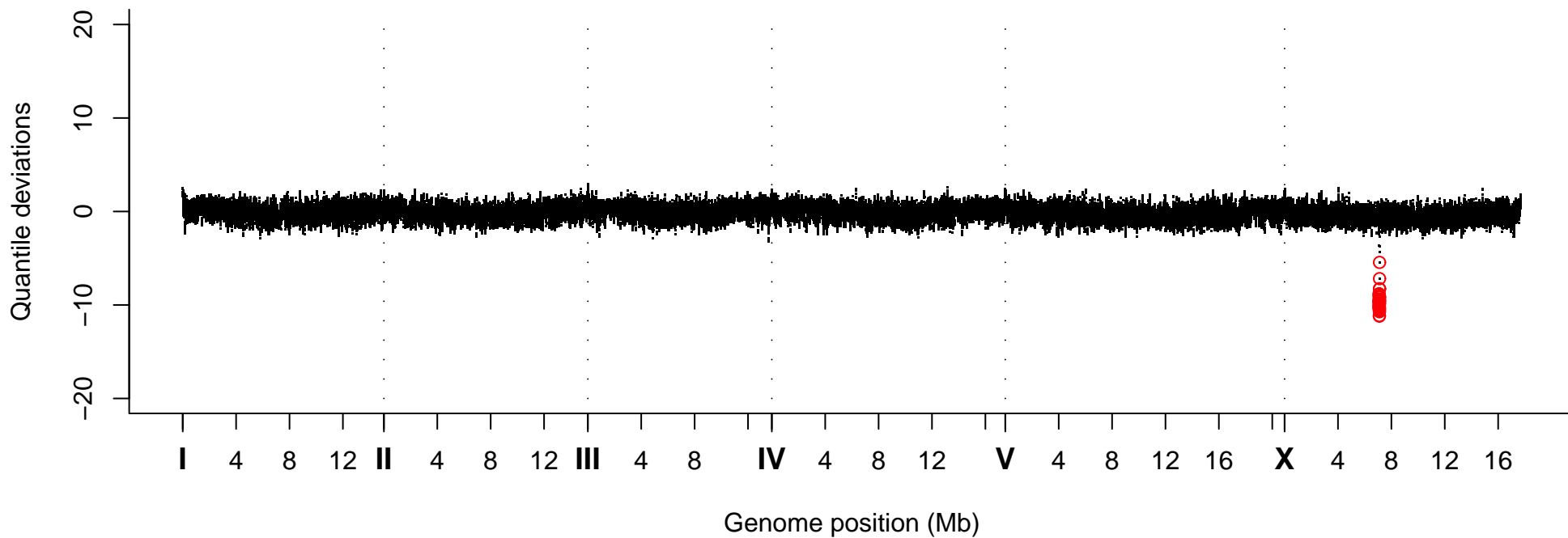
Quantile Deviations, Strain VC20766
