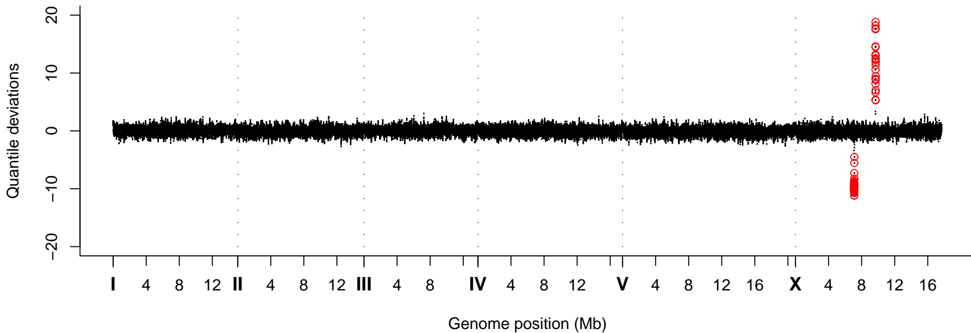
Quantile Deviations, Strain VC20771
