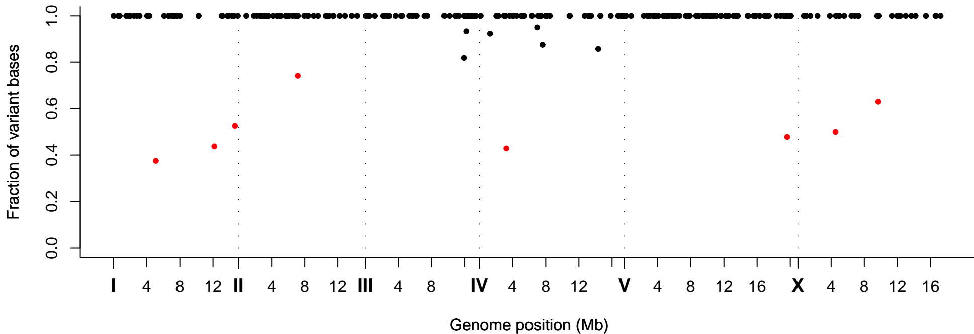
Fraction of Variant Bases at Position, Strain VC20771
