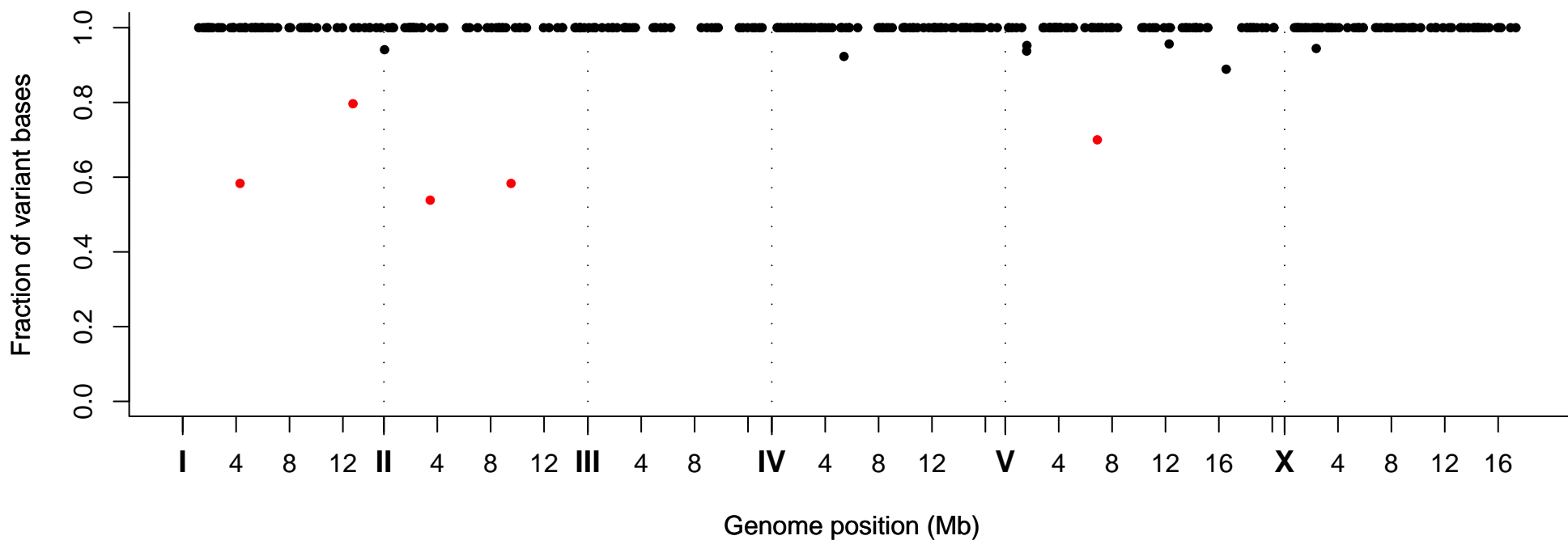
Fraction of Variant Bases at Position, Strain VC20774
