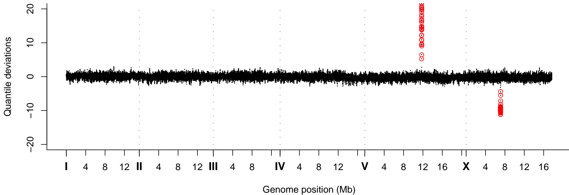
Quantile Deviations, Strain VC20774
