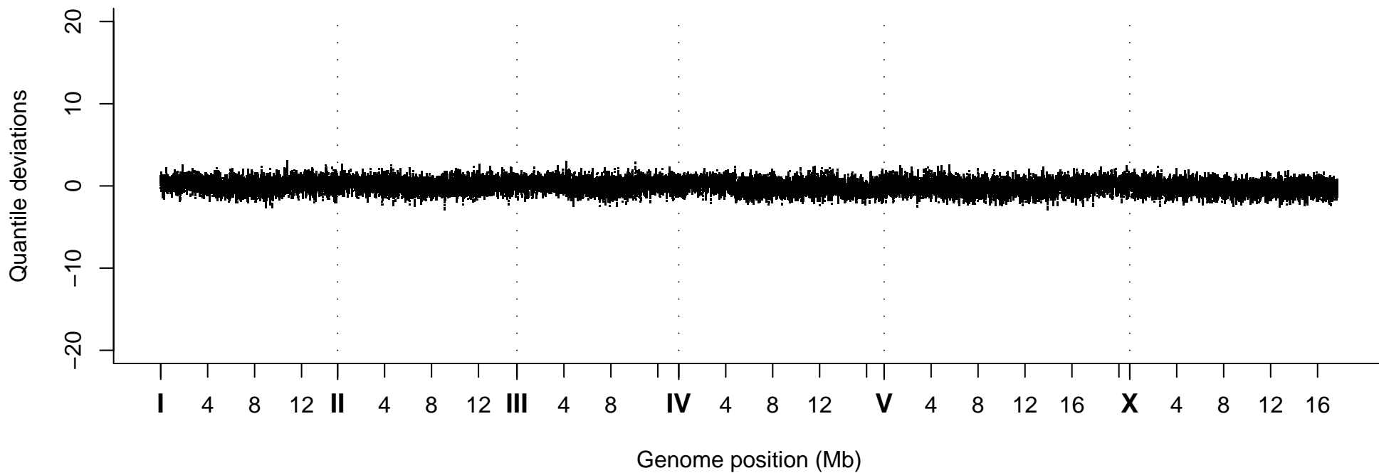
Quantile Deviations, Strain VC20777
