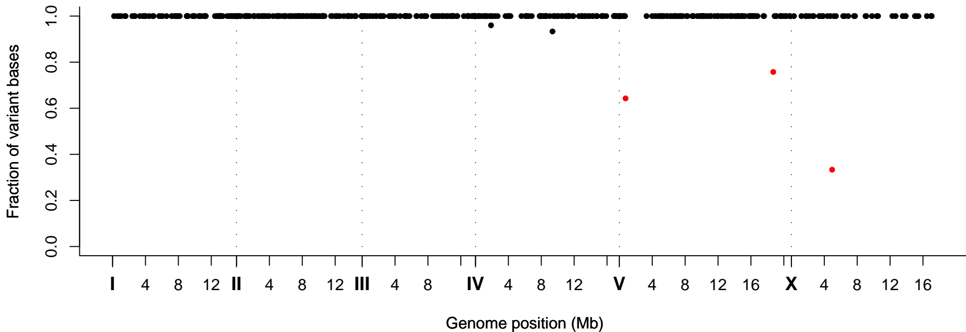
Fraction of Variant Bases at Position, Strain VC20777
