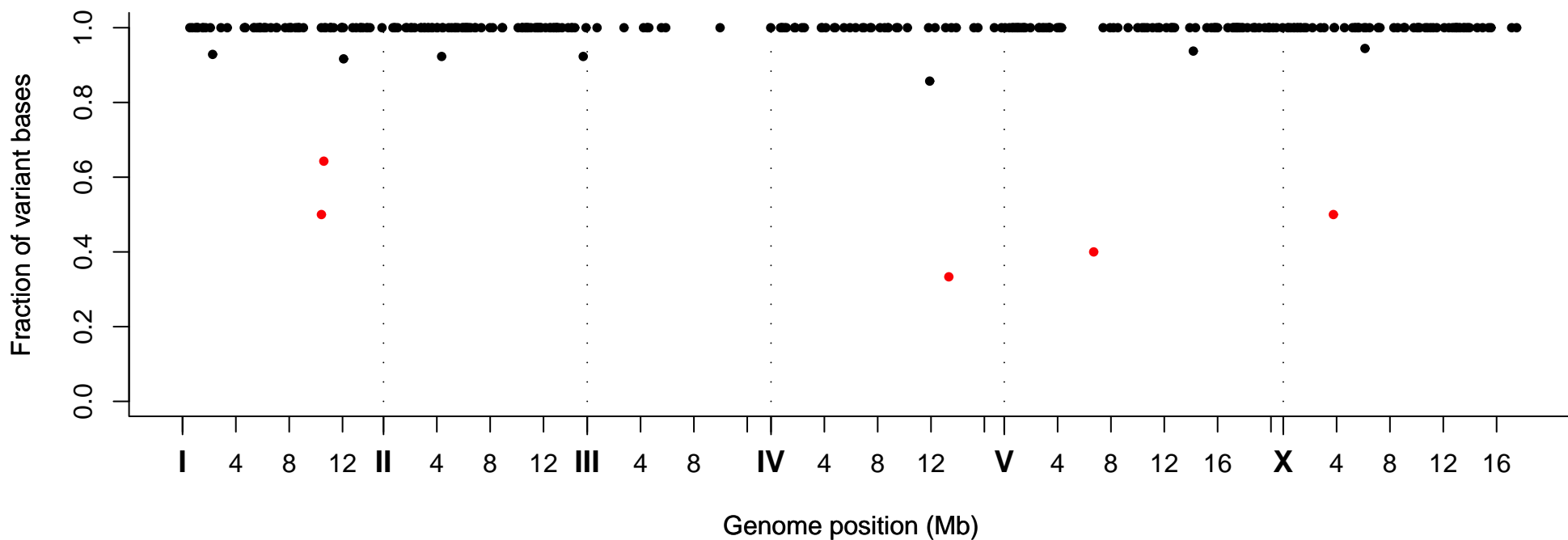
Fraction of Variant Bases at Position, Strain VC20779
