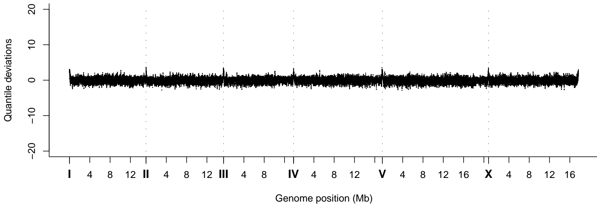
Quantile Deviations, Strain VC20779
