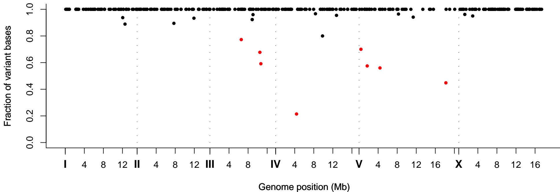
Fraction of Variant Bases at Position, Strain VC20780
