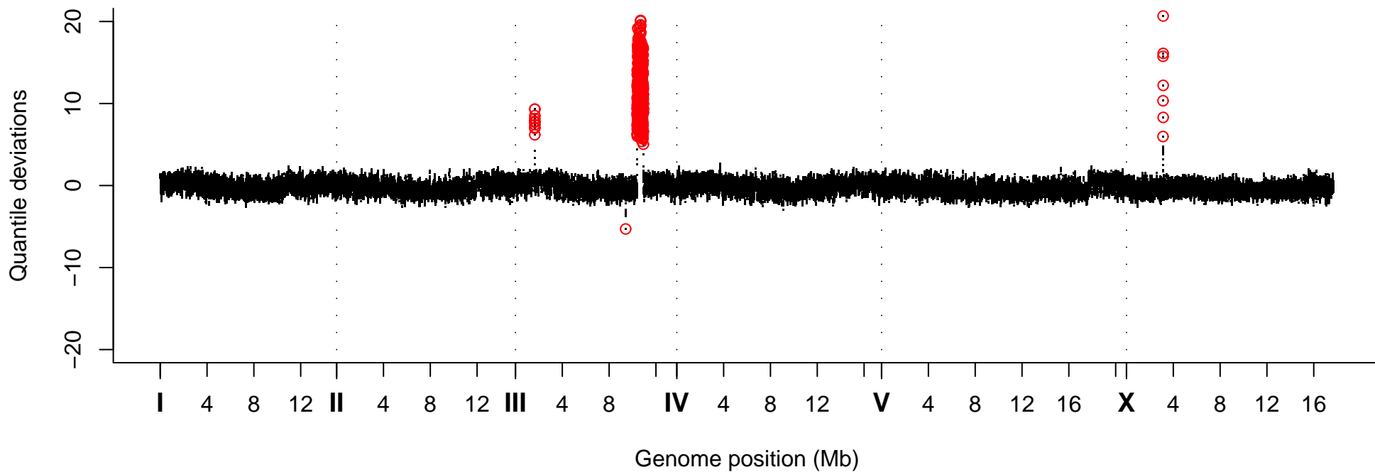
Quantile Deviations, Strain VC20780
