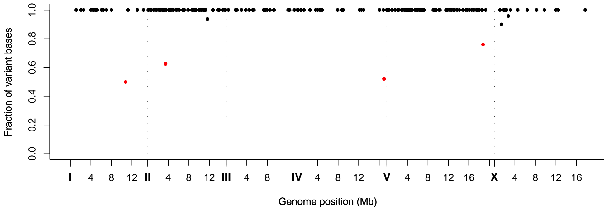
Fraction of Variant Bases at Position, Strain VC20784
