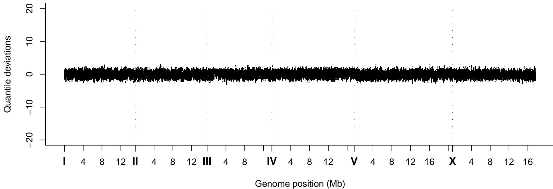
Quantile Deviations, Strain VC20784
