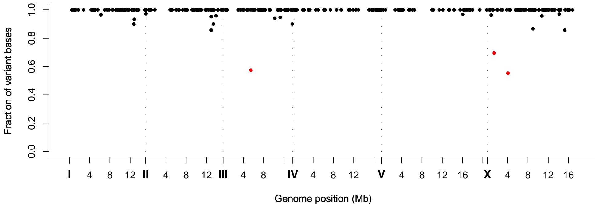
Fraction of Variant Bases at Position, Strain VC20786
