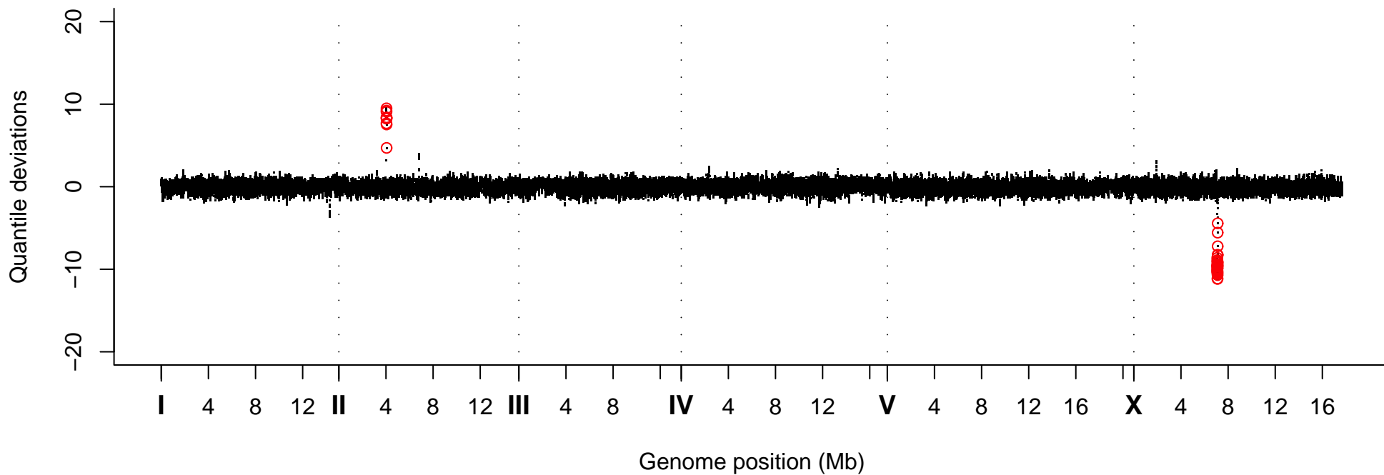
Quantile Deviations, Strain VC20786
