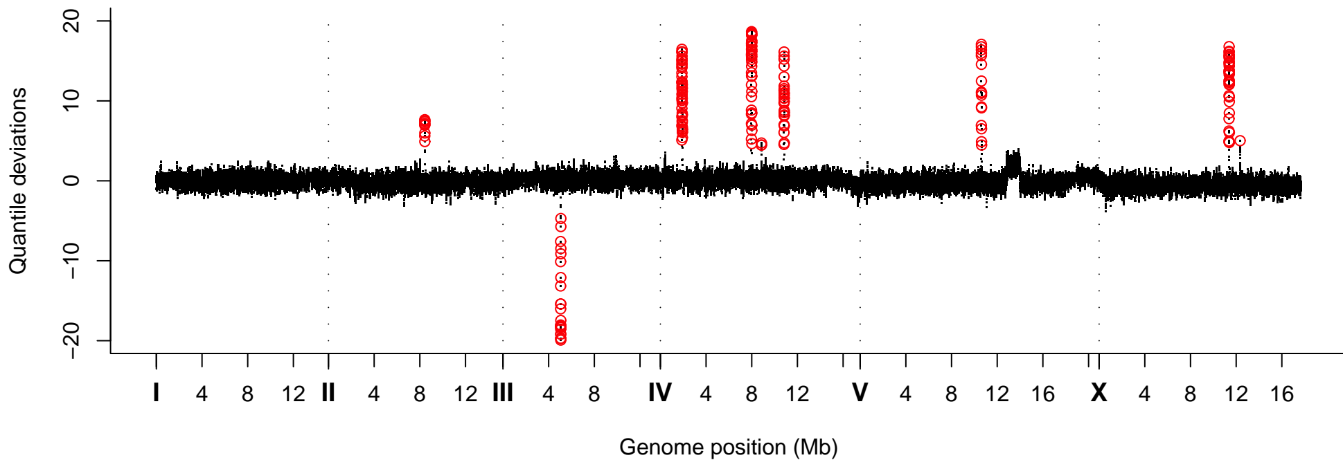
Quantile Deviations, Strain VC20791
