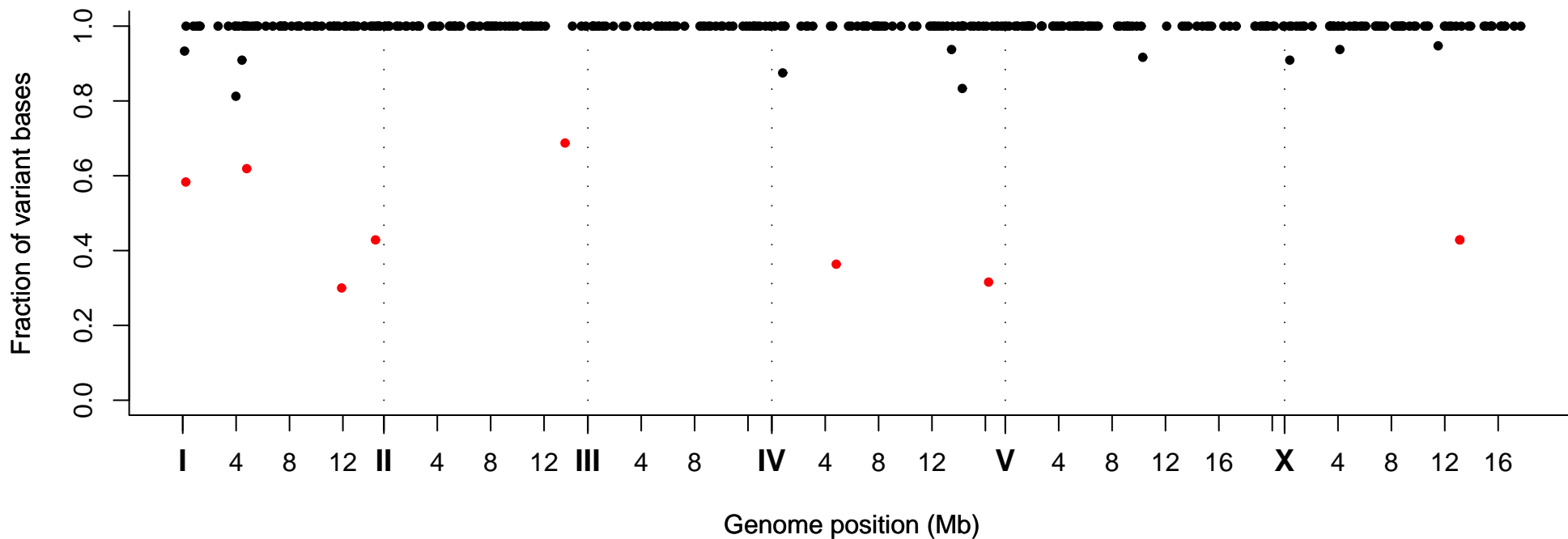
Fraction of Variant Bases at Position, Strain VC20792
