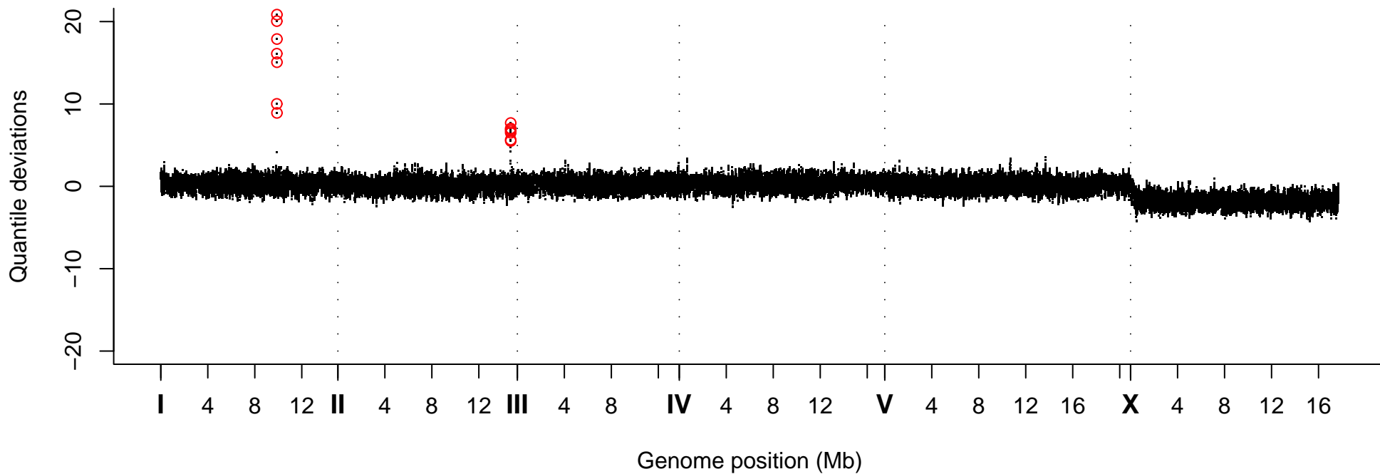
Quantile Deviations, Strain VC20792
