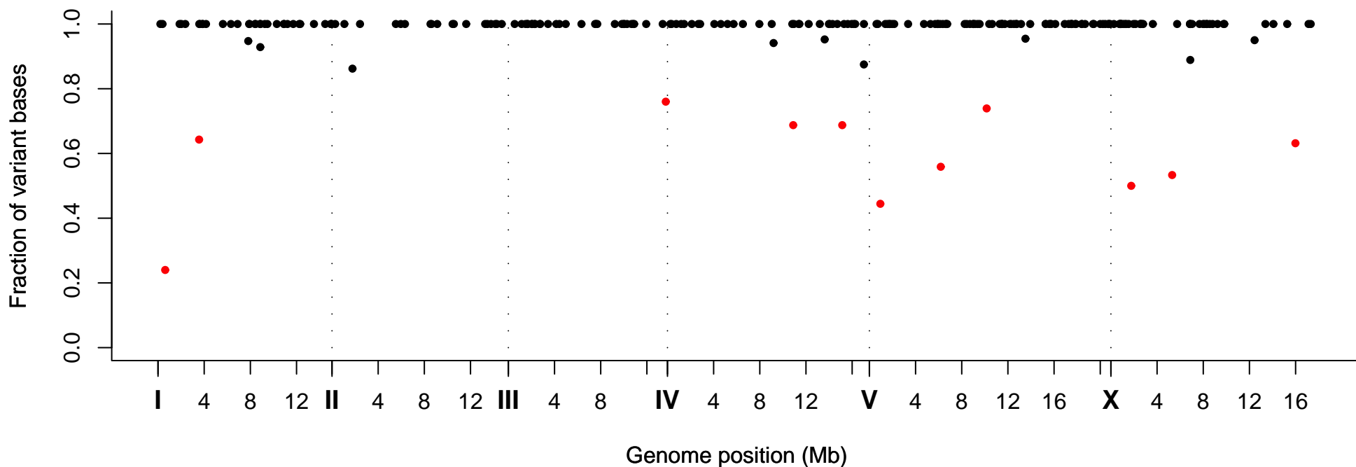
Fraction of Variant Bases at Position, Strain VC30002
