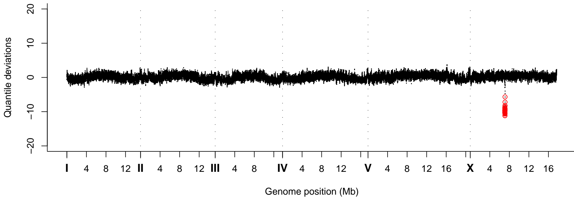
Quantile Deviations, Strain VC30002
