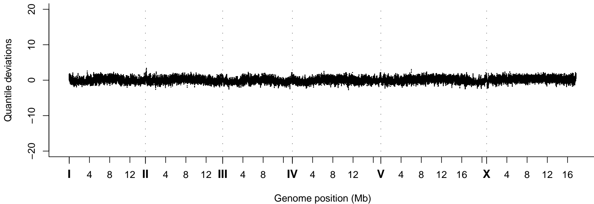
Quantile Deviations, Strain VC30004
