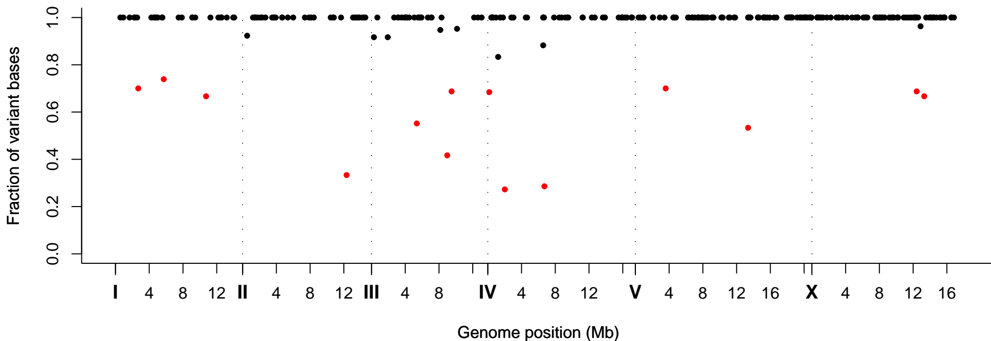
Fraction of Variant Bases at Position, Strain VC30004
