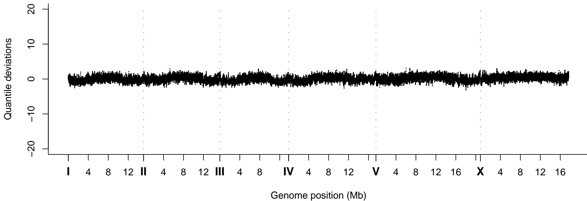
Quantile Deviations, Strain VC30005
