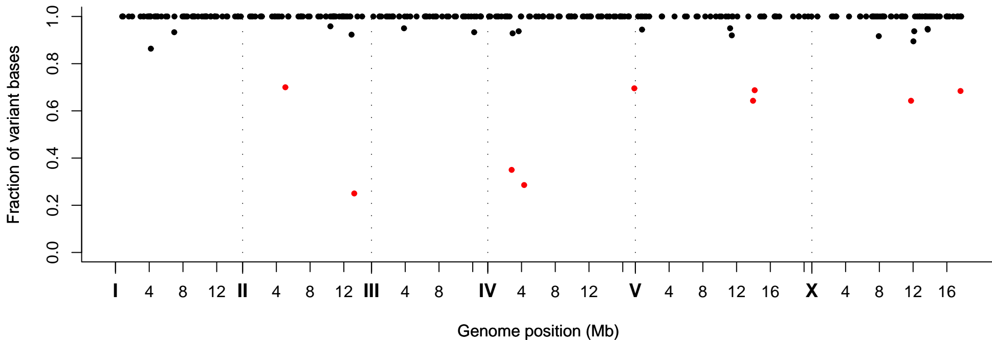
Fraction of Variant Bases at Position, Strain VC30005
