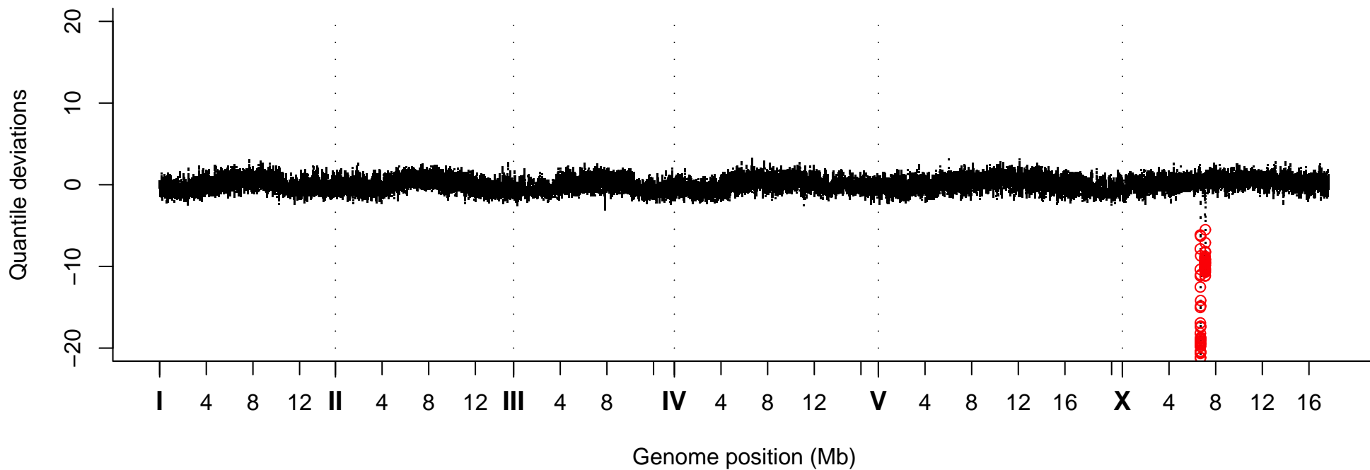
Quantile Deviations, Strain VC30006
