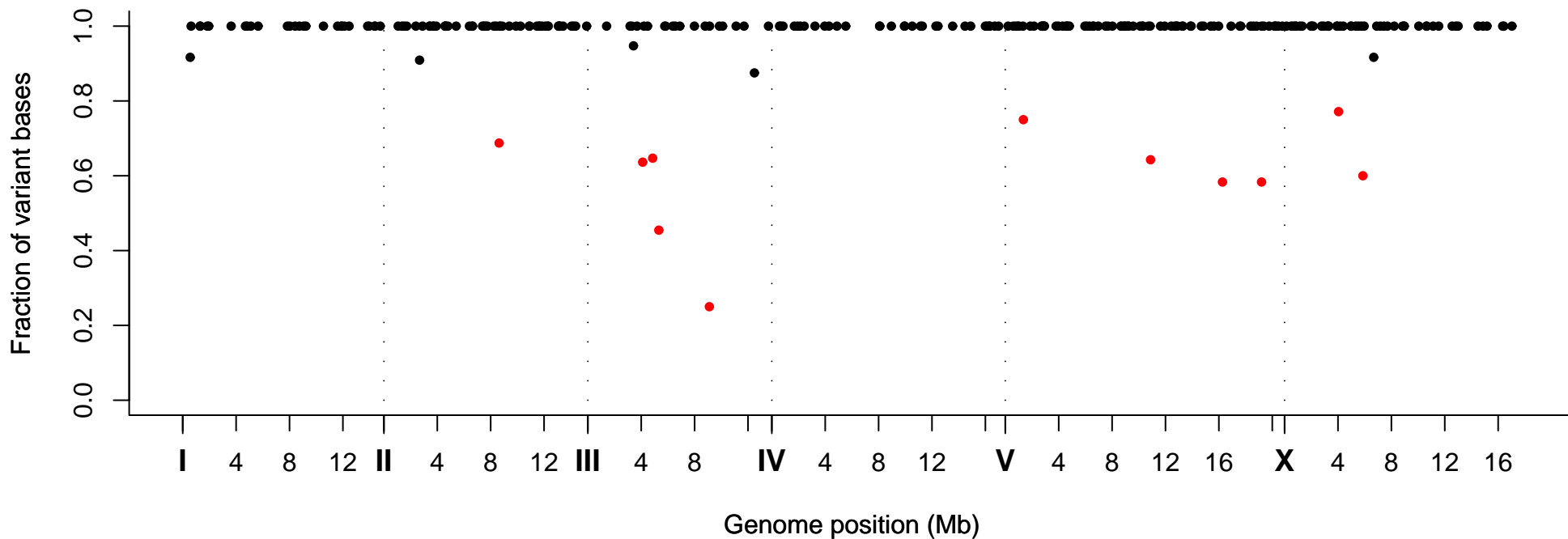
Fraction of Variant Bases at Position, Strain VC30006
