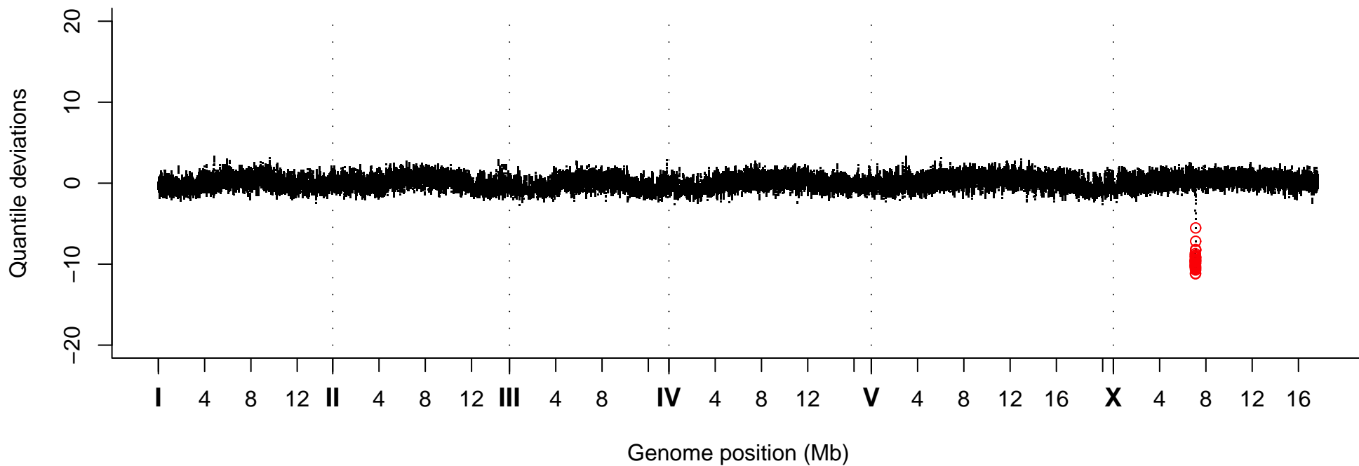
Quantile Deviations, Strain VC30007
