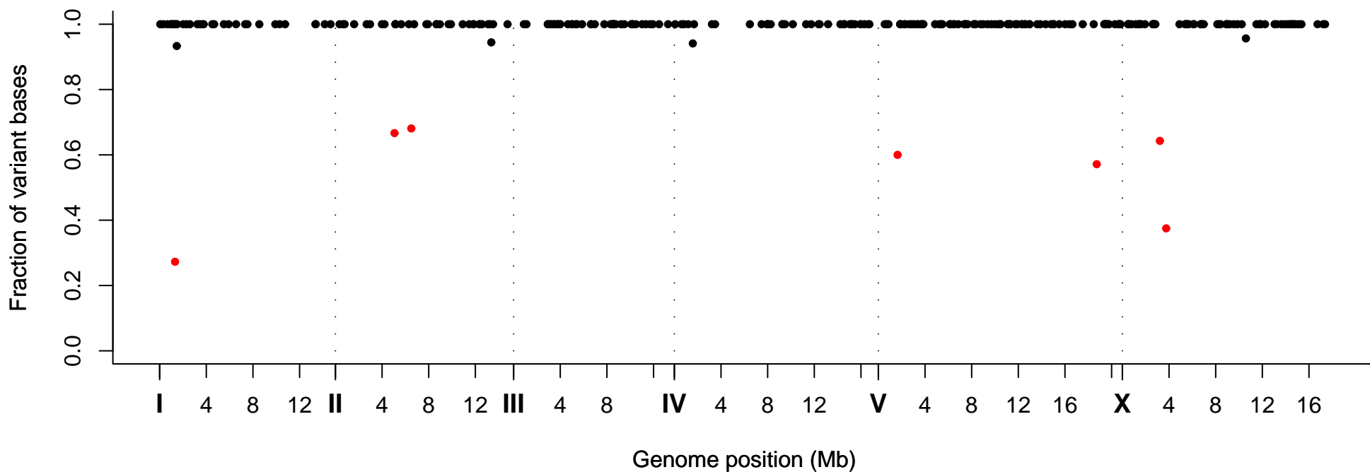
Fraction of Variant Bases at Position, Strain VC30007
