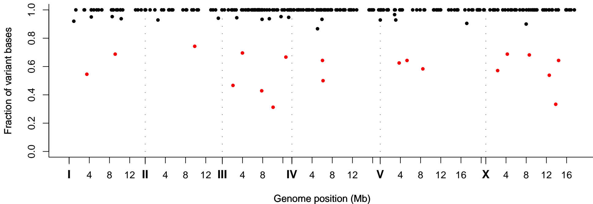
Fraction of Variant Bases at Position, Strain VC30009
