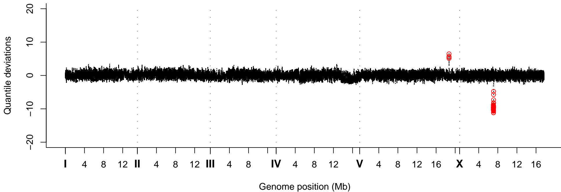
Quantile Deviations, Strain VC30009
