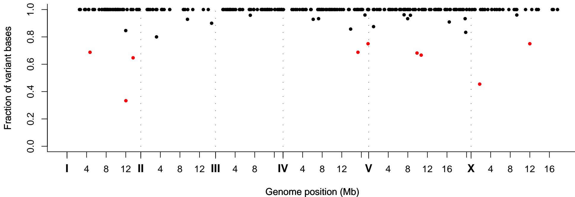
Fraction of Variant Bases at Position, Strain VC30013
