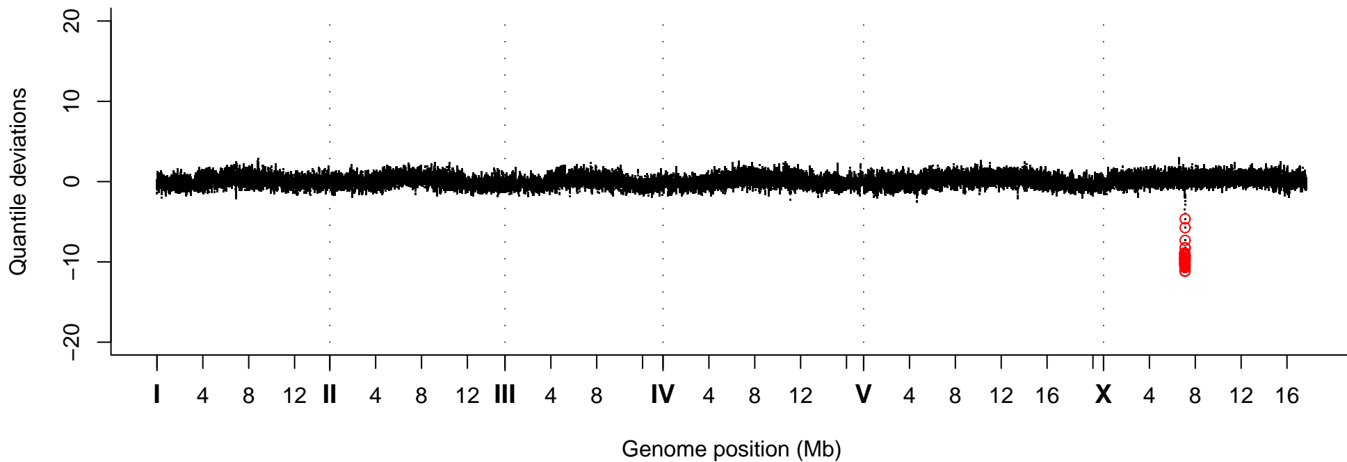
Quantile Deviations, Strain VC30013
