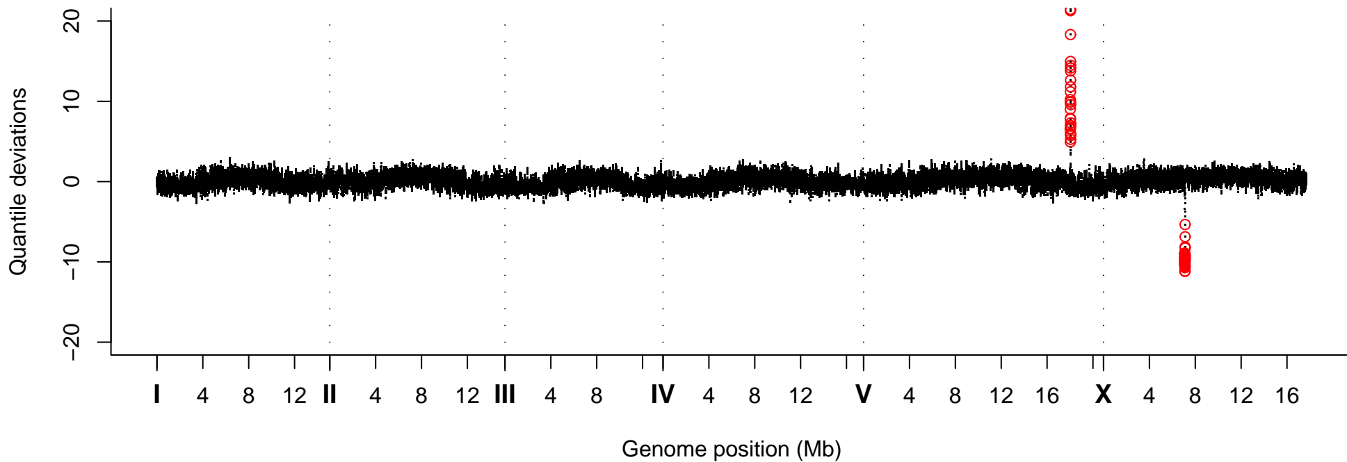
Quantile Deviations, Strain VC30015
