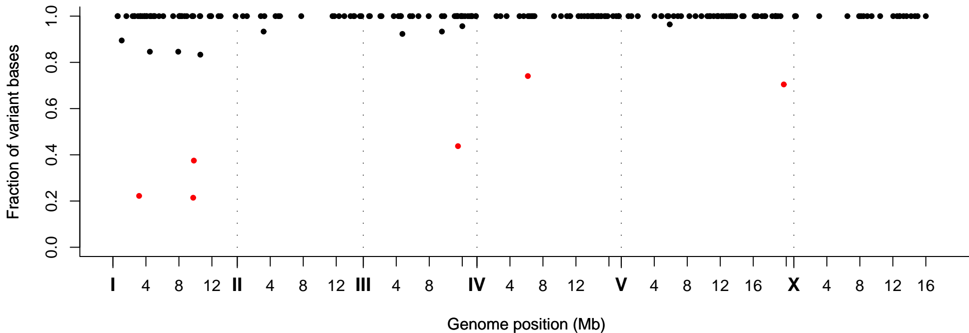
Fraction of Variant Bases at Position, Strain VC30015
