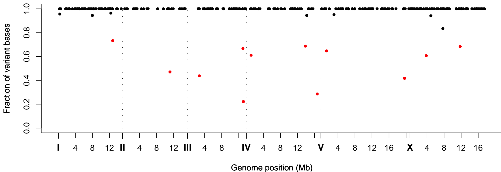
Fraction of Variant Bases at Position, Strain VC30017
