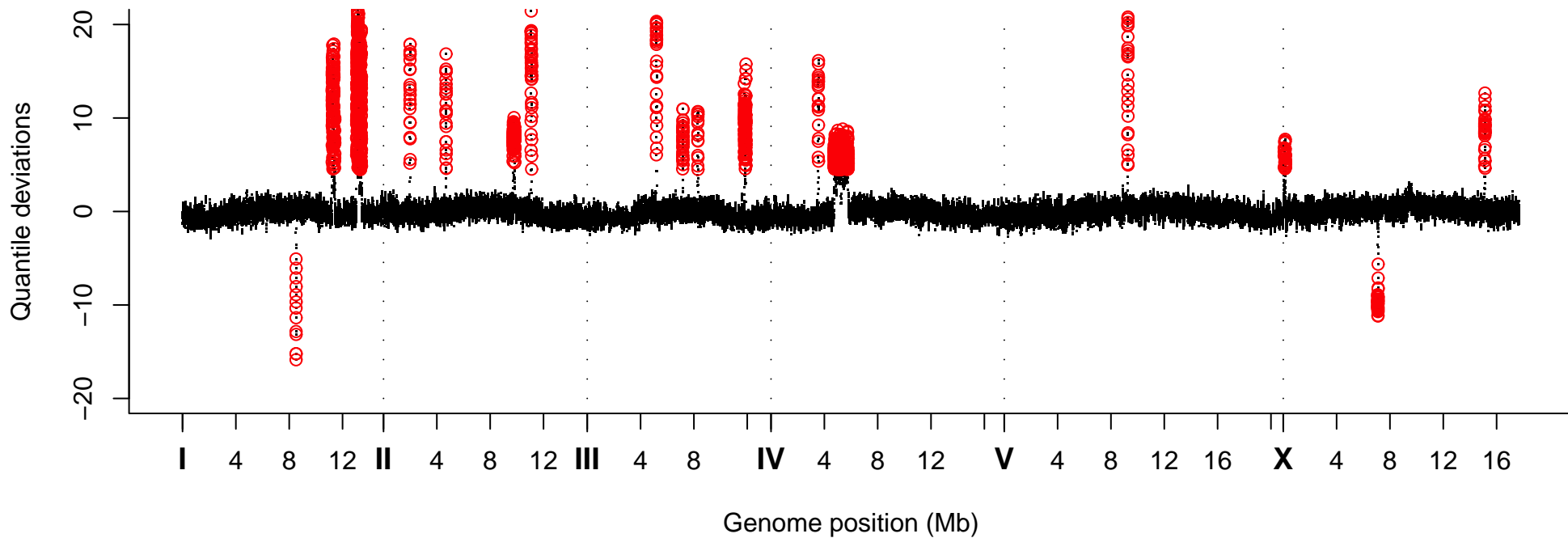
Quantile Deviations, Strain VC30017
