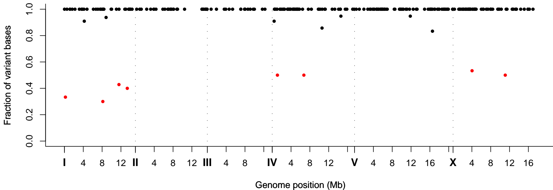
Fraction of Variant Bases at Position, Strain VC30020
