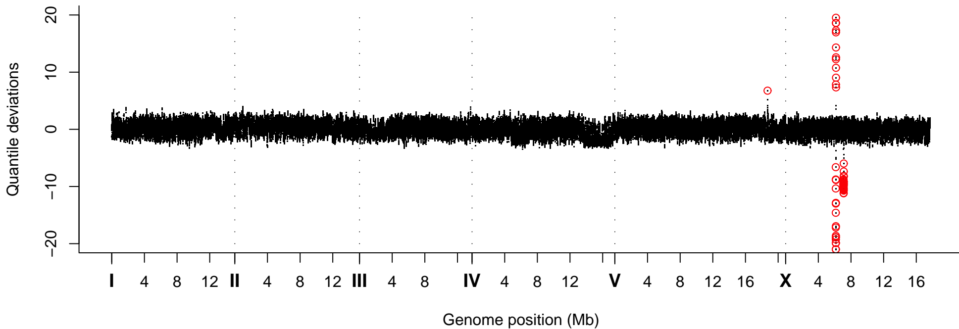
Quantile Deviations, Strain VC30020
