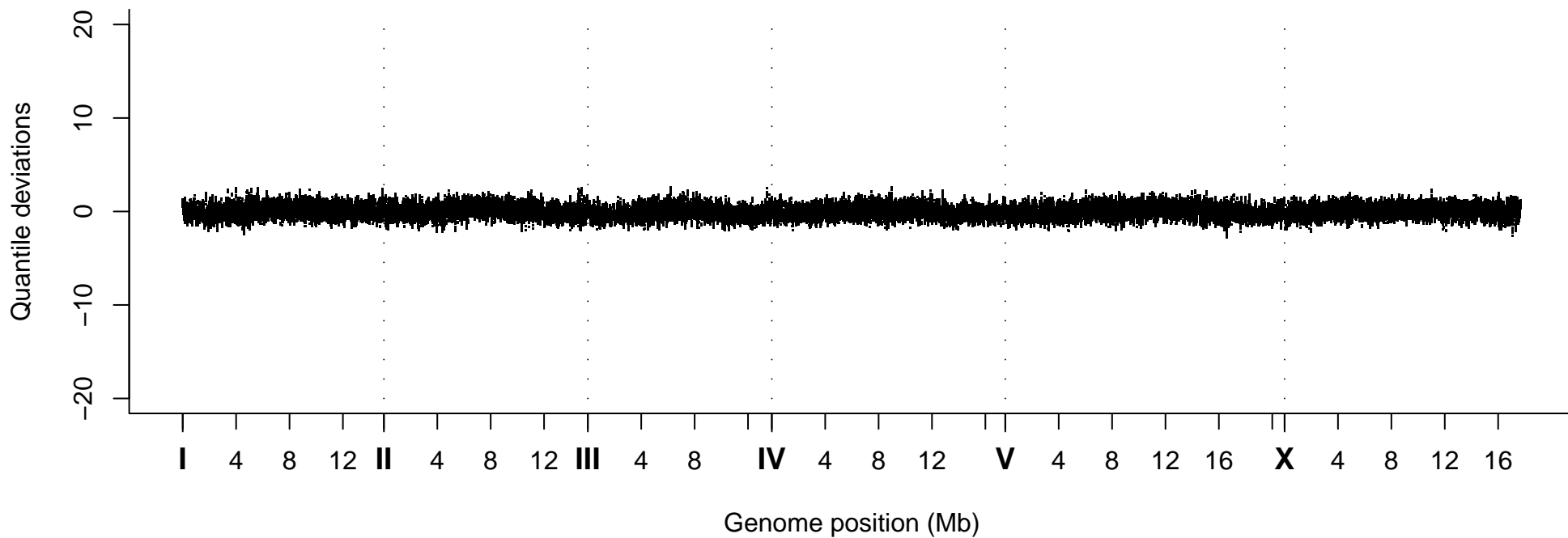
Quantile Deviations, Strain VC30021
