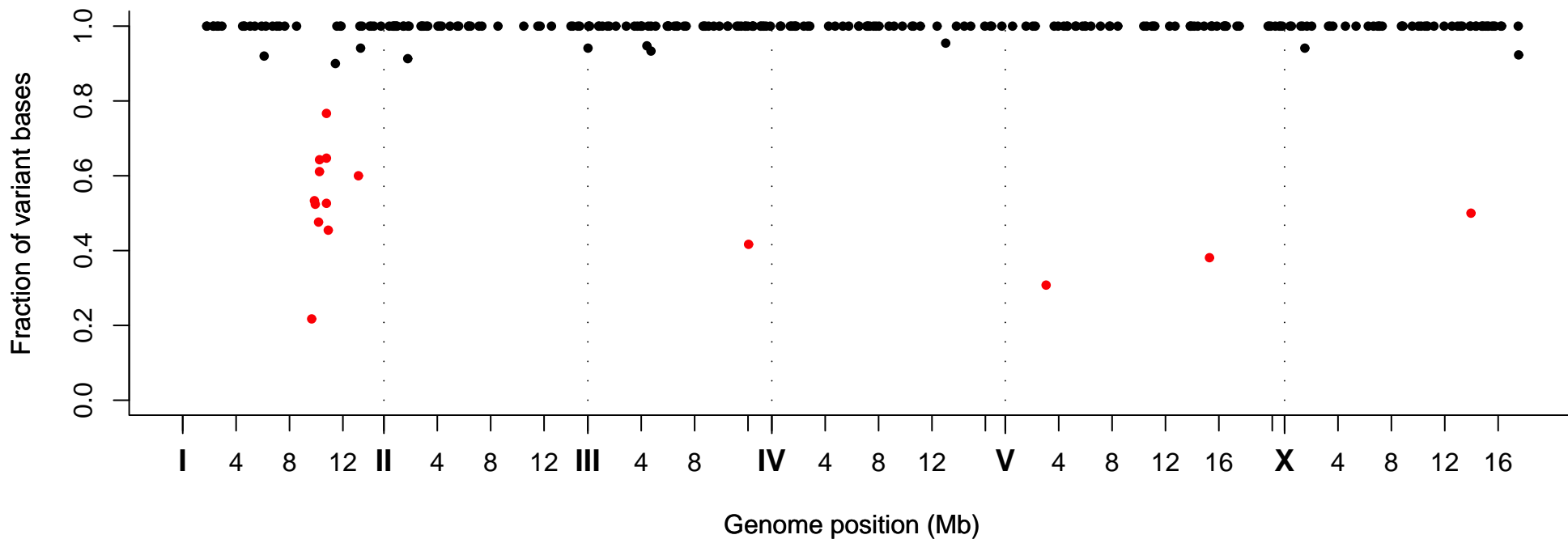
Fraction of Variant Bases at Position, Strain VC30021
