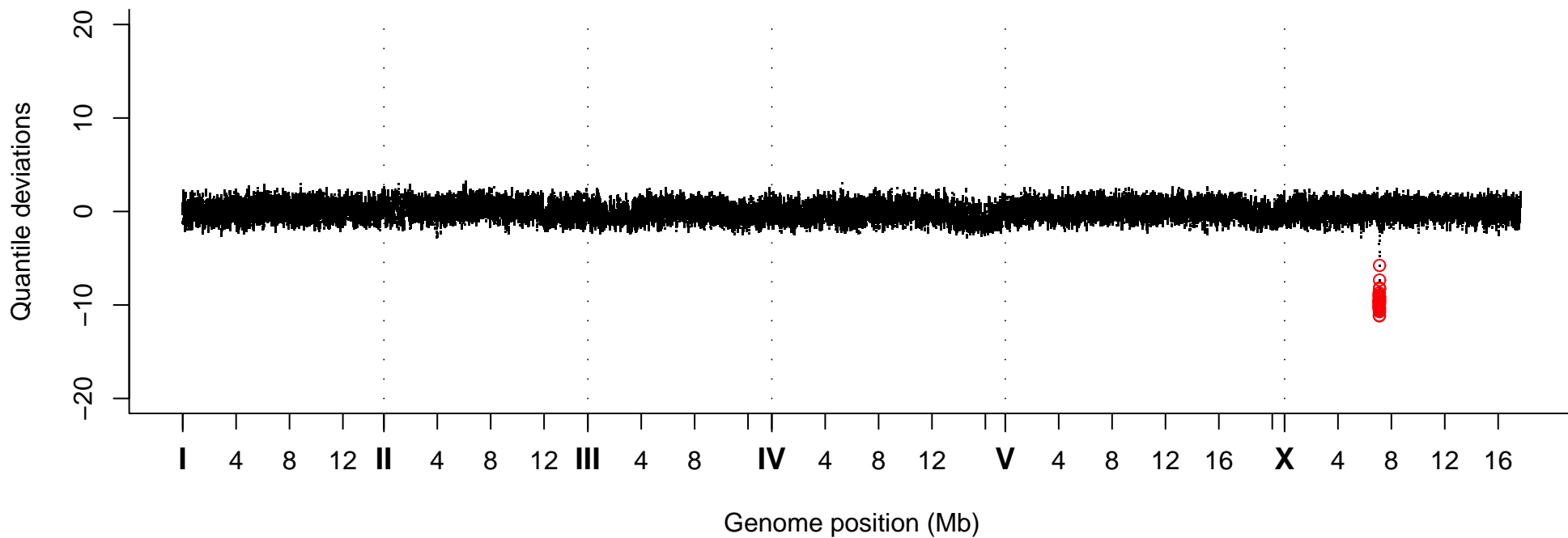
Quantile Deviations, Strain VC30022
