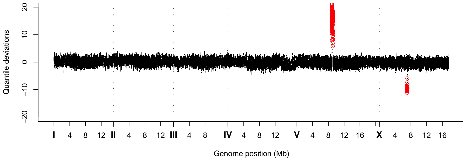
Quantile Deviations, Strain VC30023
