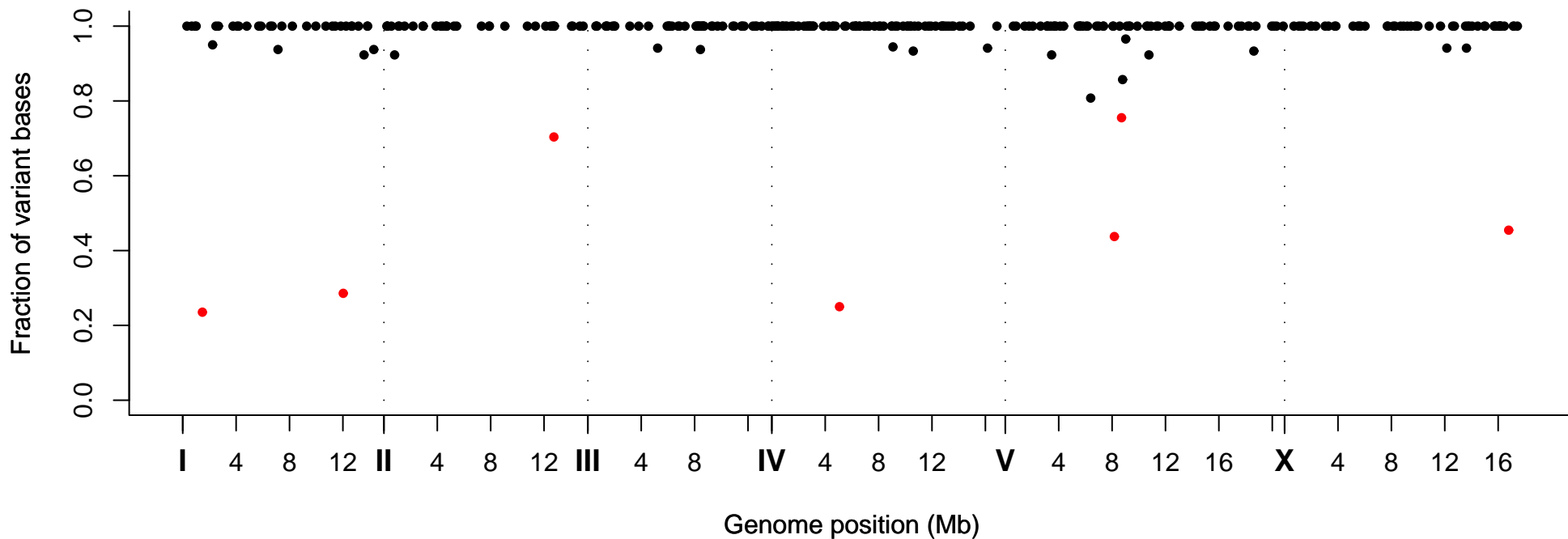
Fraction of Variant Bases at Position, Strain VC30023
