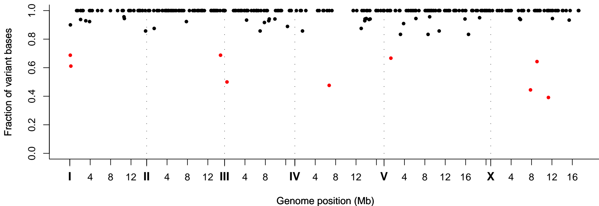
Fraction of Variant Bases at Position, Strain VC30026
