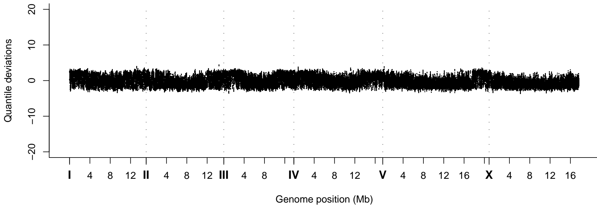
Quantile Deviations, Strain VC30026
