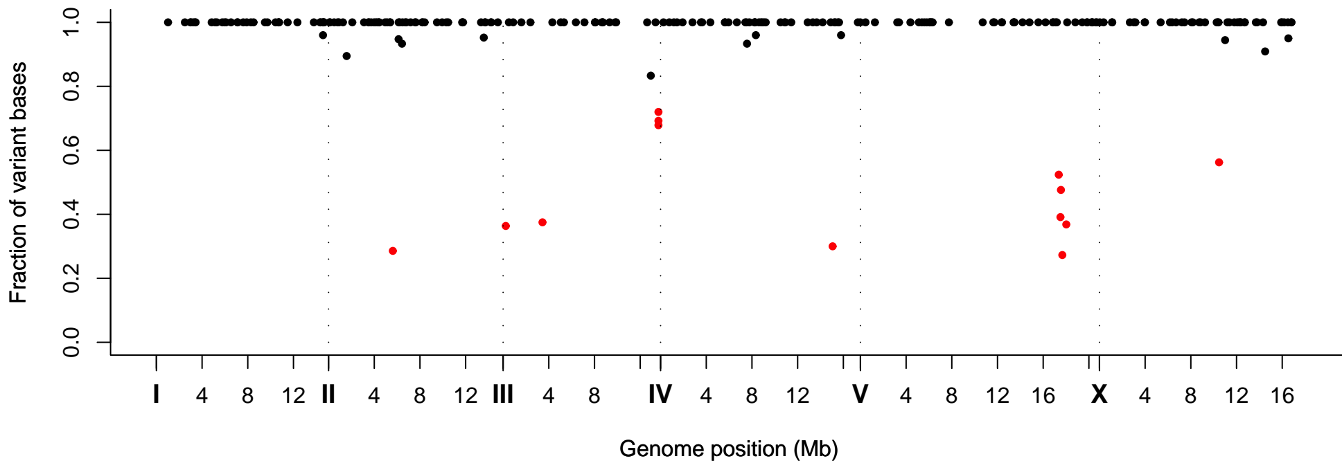
Fraction of Variant Bases at Position, Strain VC30041
