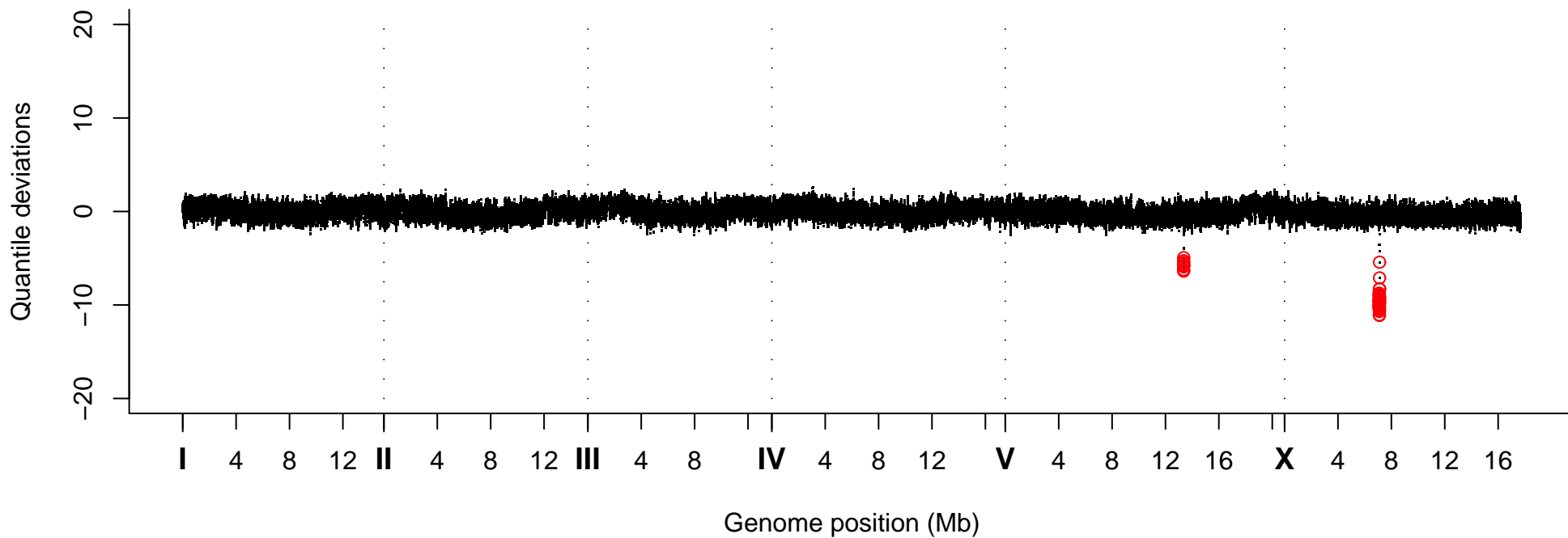
Quantile Deviations, Strain VC30041
