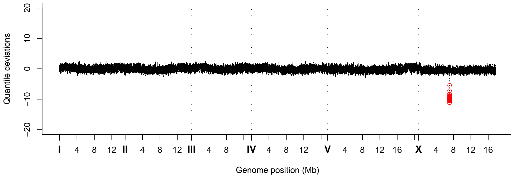
Quantile Deviations, Strain VC30042
