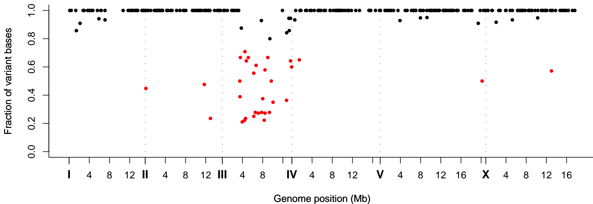
Fraction of Variant Bases at Position, Strain VC30047
