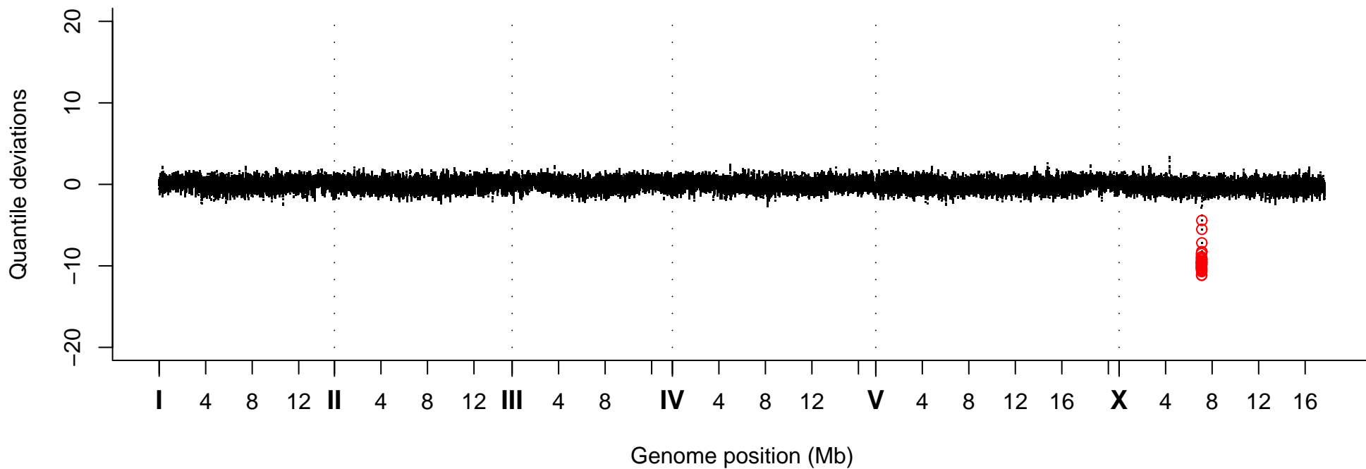
Quantile Deviations, Strain VC30047
