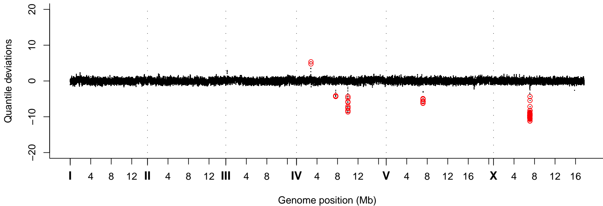
Quantile Deviations, Strain VC30055
