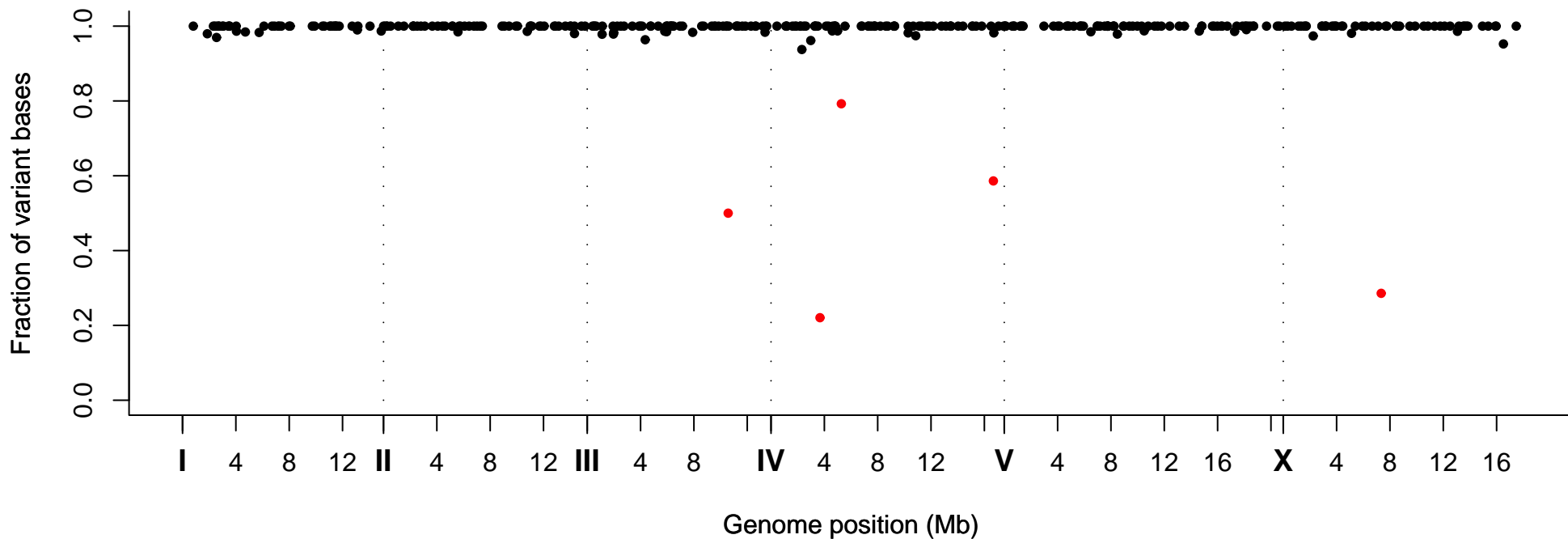
Fraction of Variant Bases at Position, Strain VC30055
