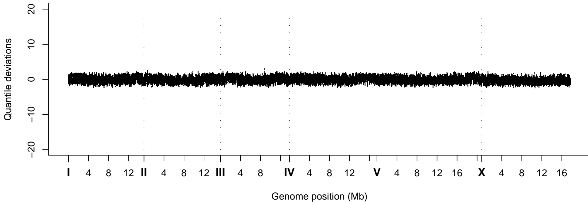
Quantile Deviations, Strain VC30058
