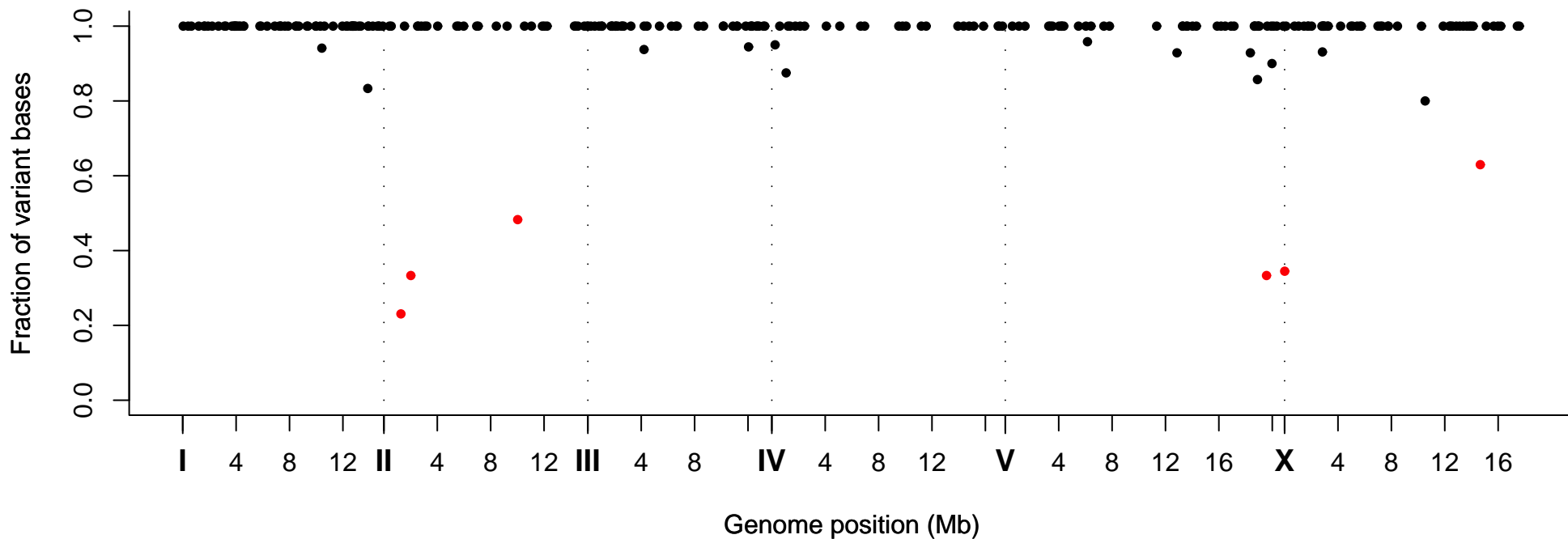
Fraction of Variant Bases at Position, Strain VC30058
