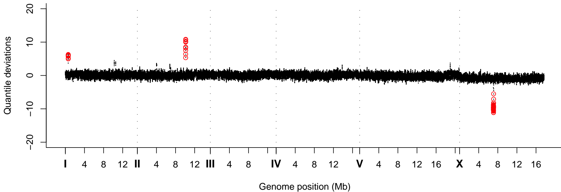
Quantile Deviations, Strain VC30060
