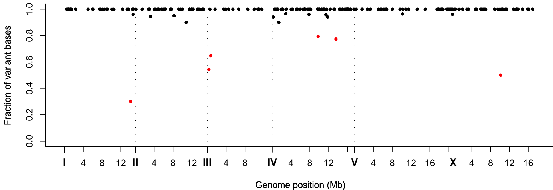
Fraction of Variant Bases at Position, Strain VC30060
