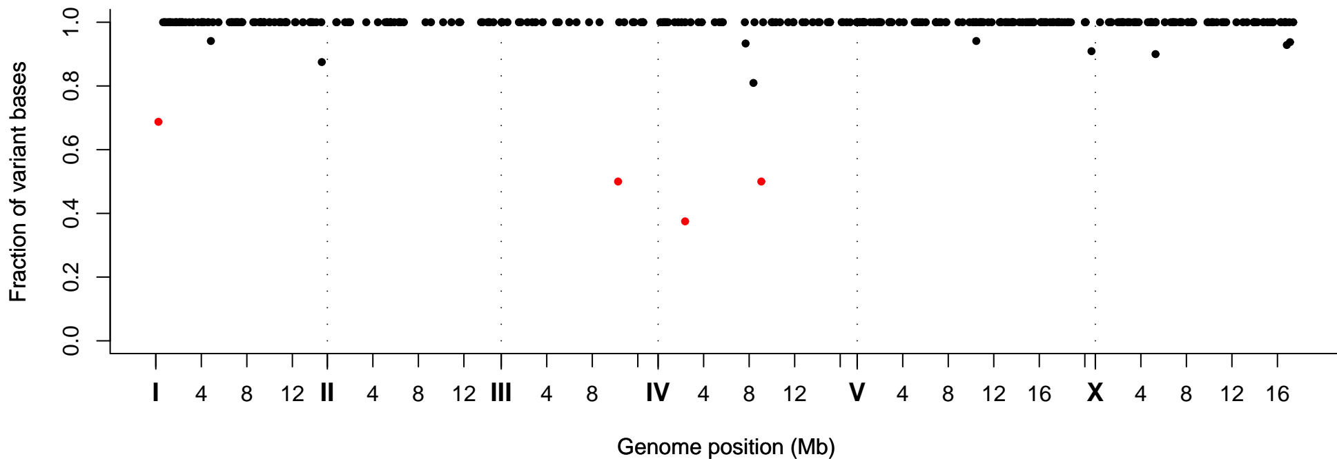
Fraction of Variant Bases at Position, Strain VC30061
