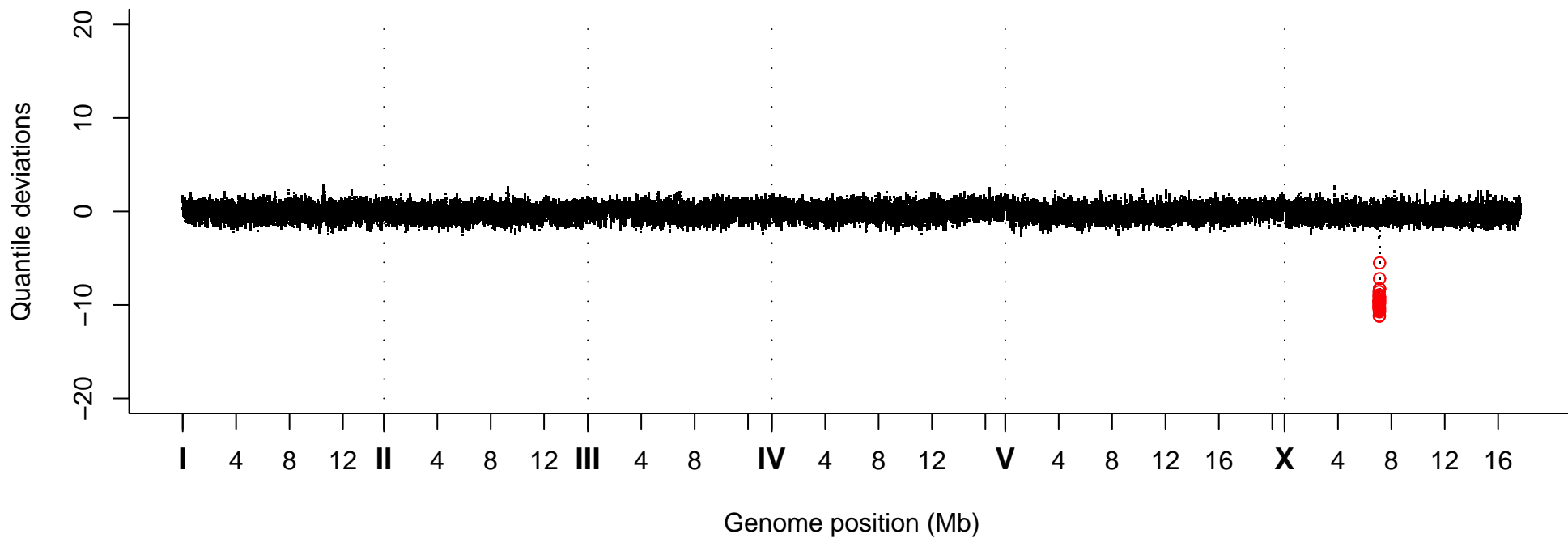
Quantile Deviations, Strain VC30061
