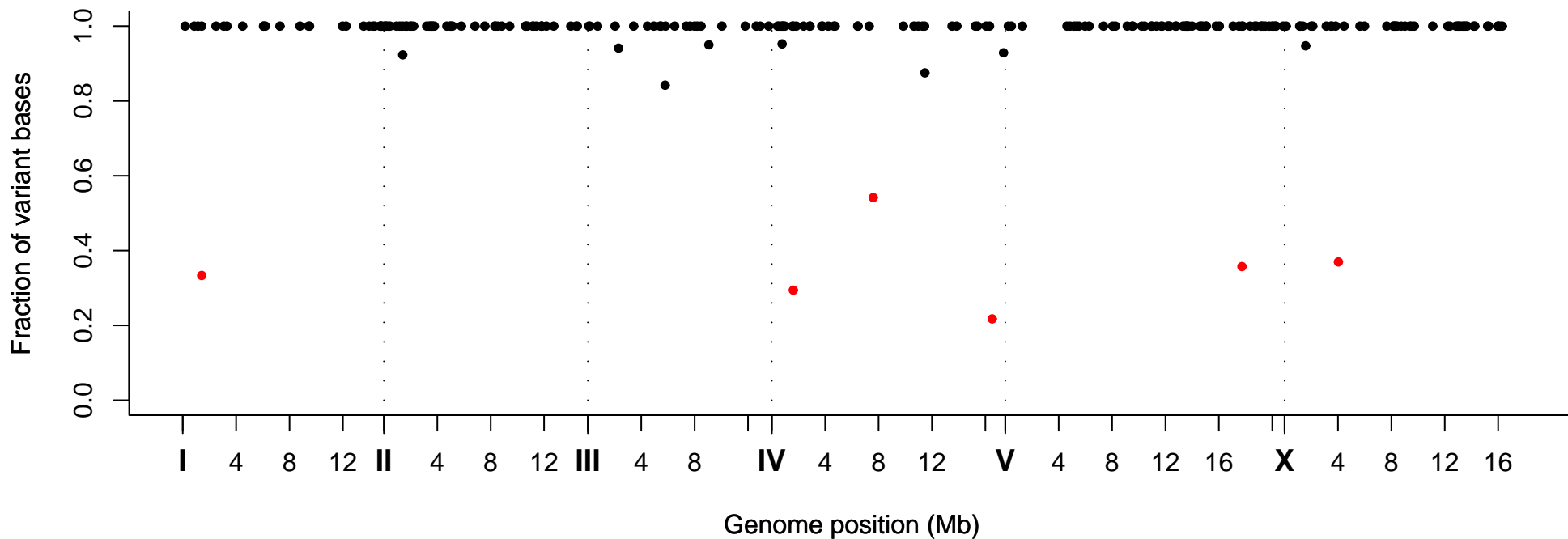
Fraction of Variant Bases at Position, Strain VC30062
