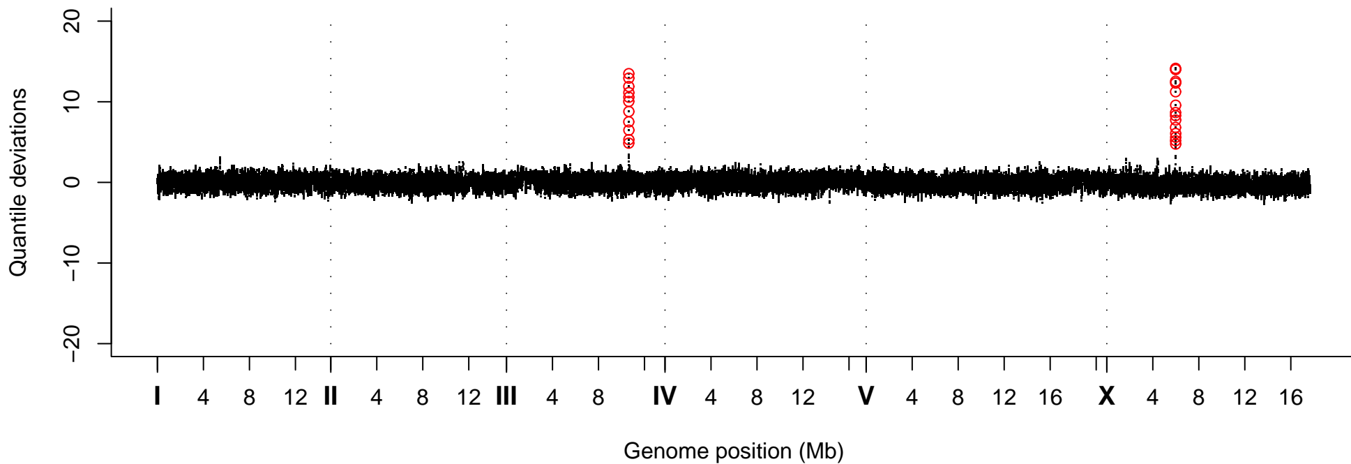
Quantile Deviations, Strain VC30062
