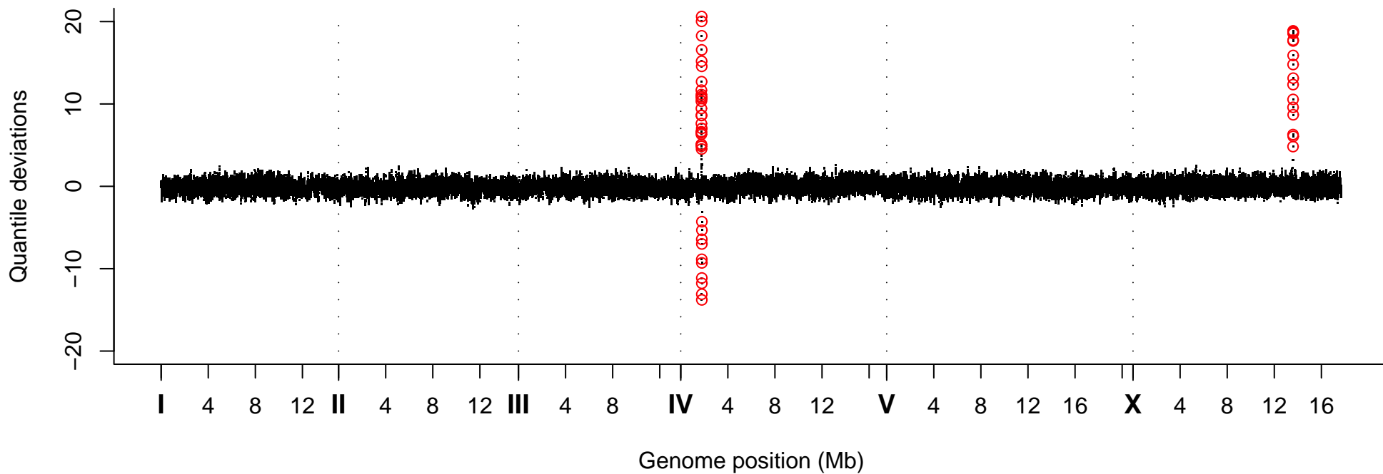
Quantile Deviations, Strain VC30076
