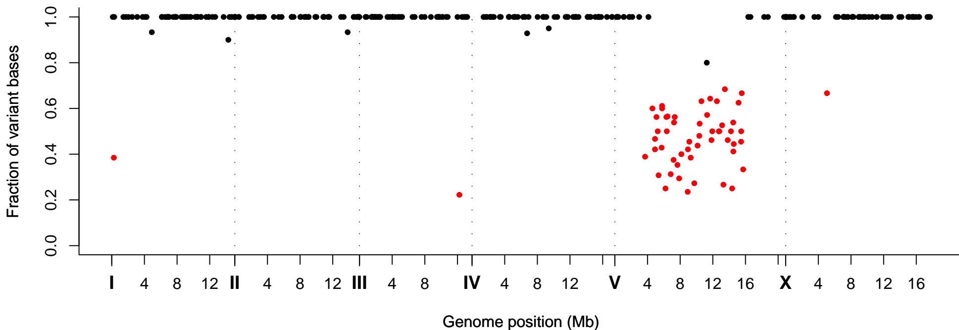
Fraction of Variant Bases at Position, Strain VC30076
