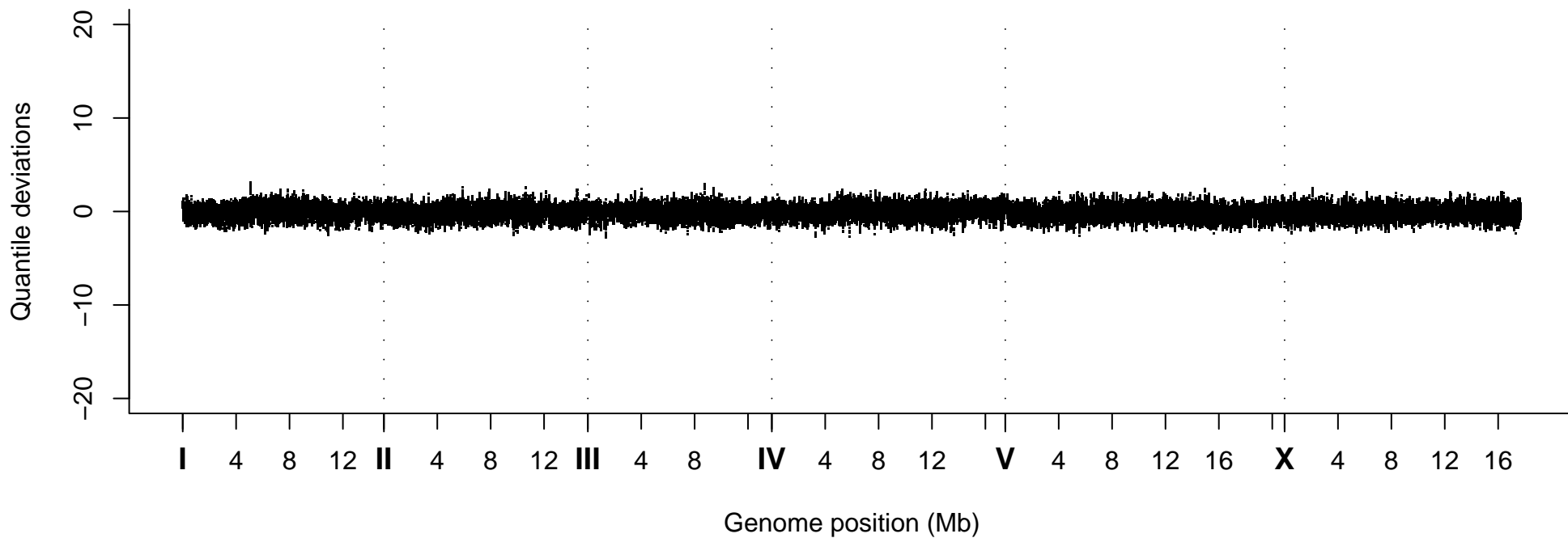
Quantile Deviations, Strain VC30090
