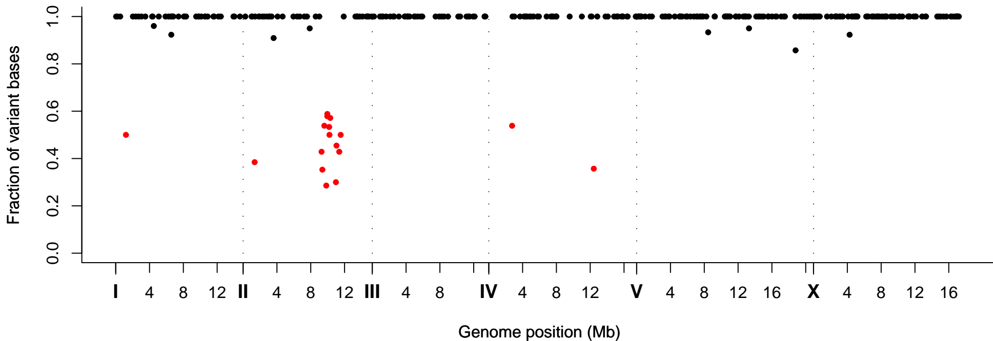
Fraction of Variant Bases at Position, Strain VC30090
