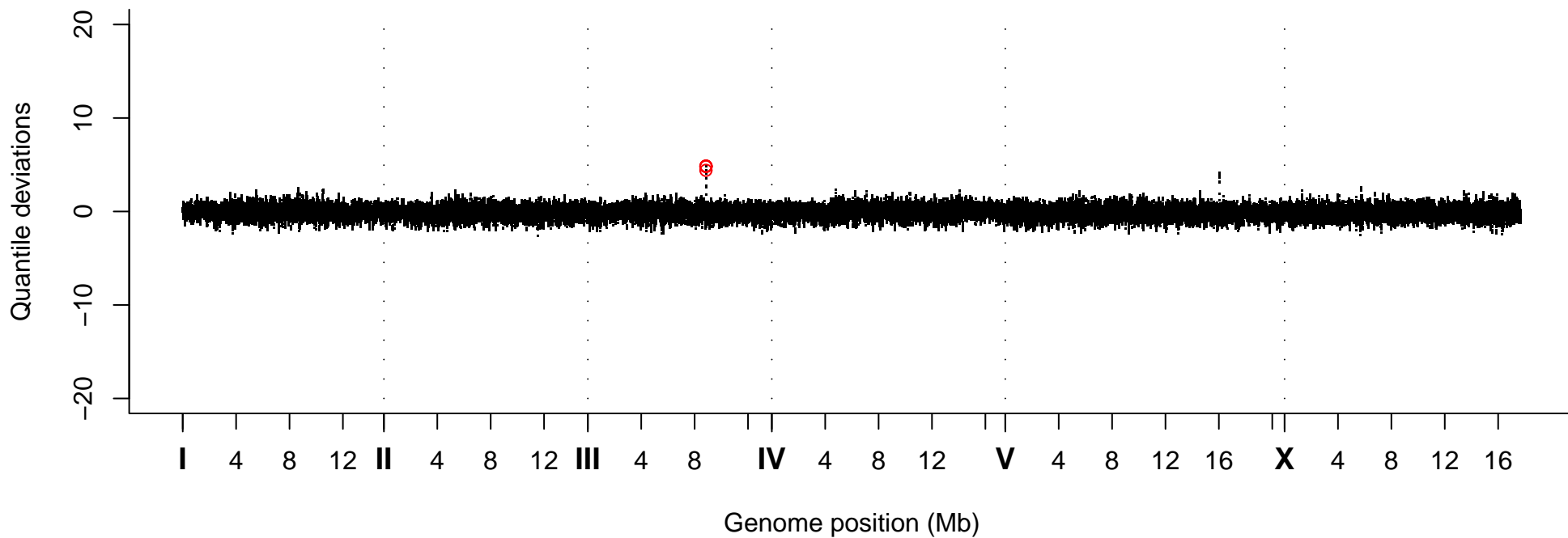
Quantile Deviations, Strain VC30091
