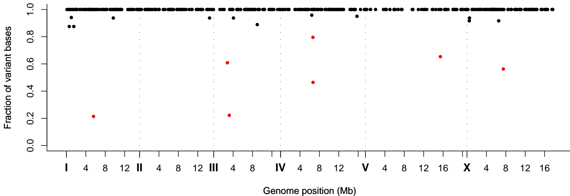
Fraction of Variant Bases at Position, Strain VC30091
